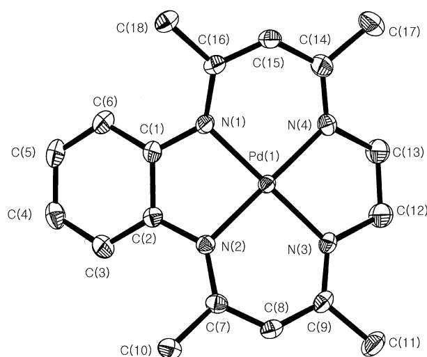
Figure 3. The molecular structure of palladium(II) complex.
