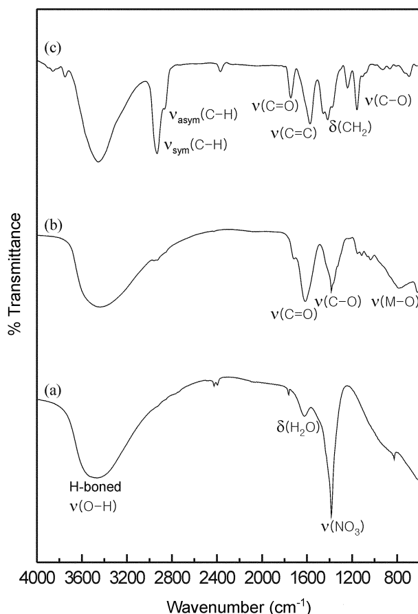
Figure 3. Infrared spectra for (a) Zn 3 Al(NO 3 ) 2 -LDH, (b) Zn 2 Al(vitamin C)-LDH, and (c) Zn 3 Al(vitamin E)-LDH.
