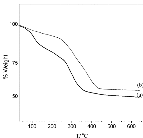
Figure 4. TGA profiles for (a) Zn 2 Al(vitamin C)-LDH and (b) Zn 2 Al(vitamin E)-LDH.
