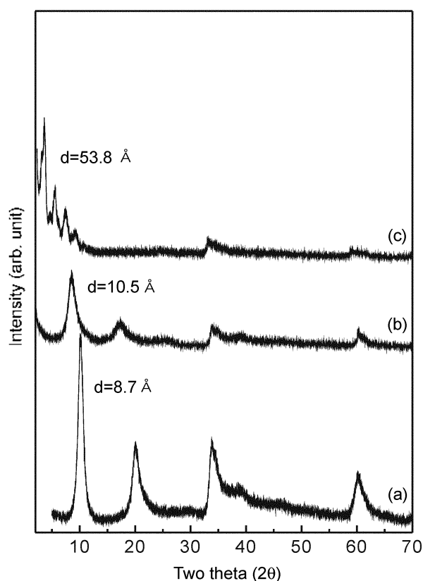
Figure 2. Powder X-ray diffraction patterns for (a) Zn 3 Al(NO 3 )-LDH, (b) Zn 2 Al(vitamin C)-LDH and (c) Zn 3 Al(vitamin E)-LDH.
