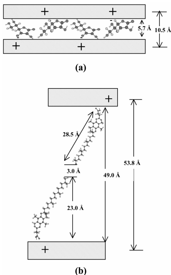
Figure 6. Schematic illustrations of (a) Zn_3Al (vitamin C)-LDH, and (b) Zn_2Al (vitamin E)-LDH.
