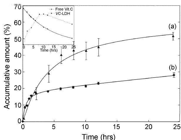
Figure 7. Release patterns of intercalated (a) vitamin C and (b) vitamin E. Inlet shows that free vitamin C (solid) and deintercalated vitamin C (dot).
