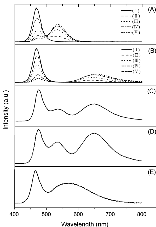
Figure 2. (A, B) Photoluminescence spectra of (A) blue- and green-emitting LEDs, and (B) blue- and red-emitting LEDs, where \text{SrGa}_2\text{S}_4:\text{Eu} (green) or \text{SrY}_2\text{S}_4:\text{Eu} (red) phosphor films are coated to a blue LED. No phosphor is used in (I). The amount of phosphor increases on going from (II) to (V). (C, D) Photoluminescence spectra of three-band white LEDs with color temperatures of (C) 5620 K and (D) 4550 K, where the ratio of \text{SrGa}_2\text{S}_4:\text{Eu} to \text{SrY}_2\text{S}_4:\text{Eu} is fixed at 0.2, and larger amounts of the phosphors are used in (D). (E) Photoluminescence spectrum of a two-band white LED with a color temperature of 5240 K in which the (\text{Y}_{0.6}\text{Gd}_{0.4})_2\text{Al}_3\text{O}_{12}:\text{Ce}_{0.3} (yellow) phosphor was used.
