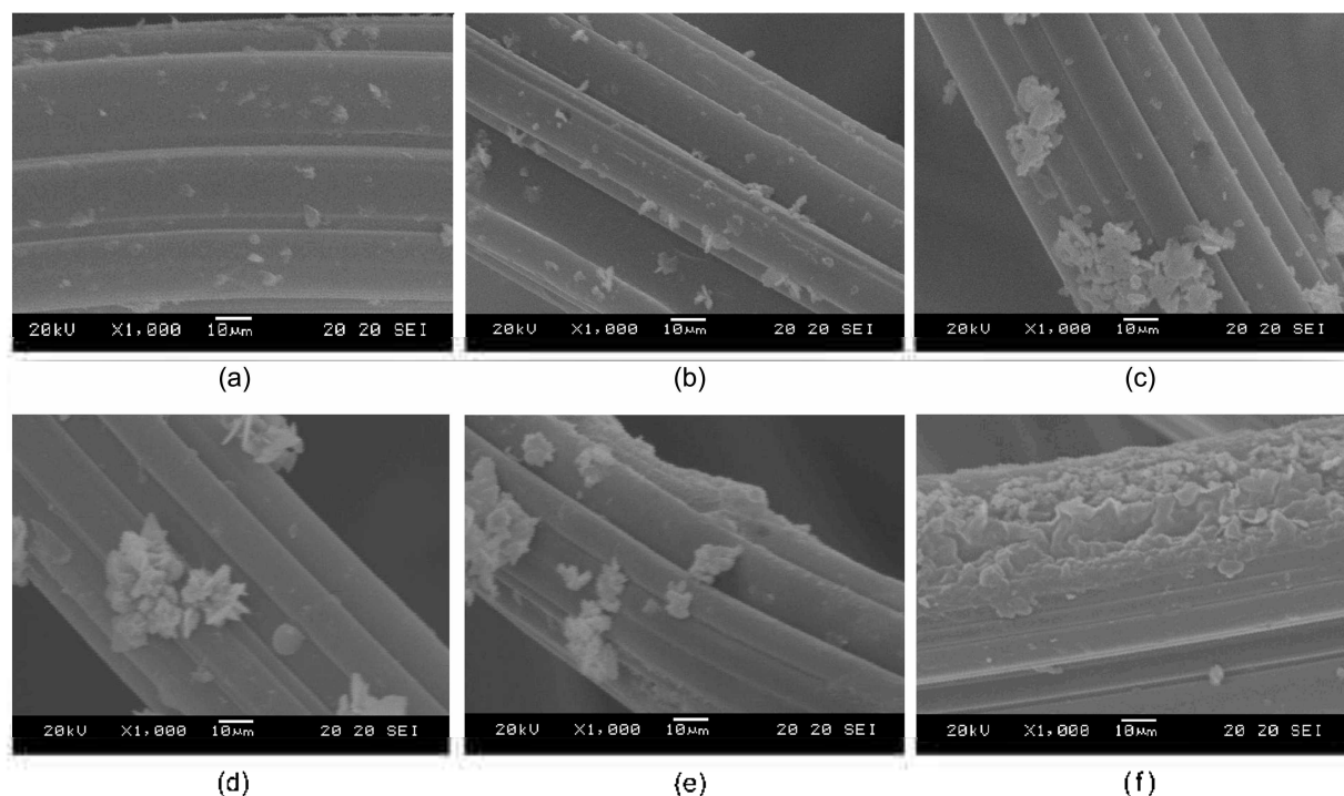
Figure 3. SEM micrographs of acid free metallic silver supported activated carbon fiber and metallic silver supported activated carbon fibers after sulfuric acid treatments: (a) \text{Ag}_{0.1}\text{-ACF} . (b) 0.01\text{H}_2\text{SO}_4\text{-Ag}_{0.1}\text{-ACF} . (c) 0.03\text{H}_2\text{SO}_4\text{-Ag}_{0.1}\text{-ACF} . (d) 0.05\text{H}_2\text{SO}_4\text{-Ag}_{0.1}\text{-ACF} . (e) 0.07\text{H}_2\text{SO}_4\text{-Ag}_{0.1}\text{-ACF} and (f) 0.1\text{H}_2\text{SO}_4\text{-Ag}_{0.1}\text{-ACF} .
