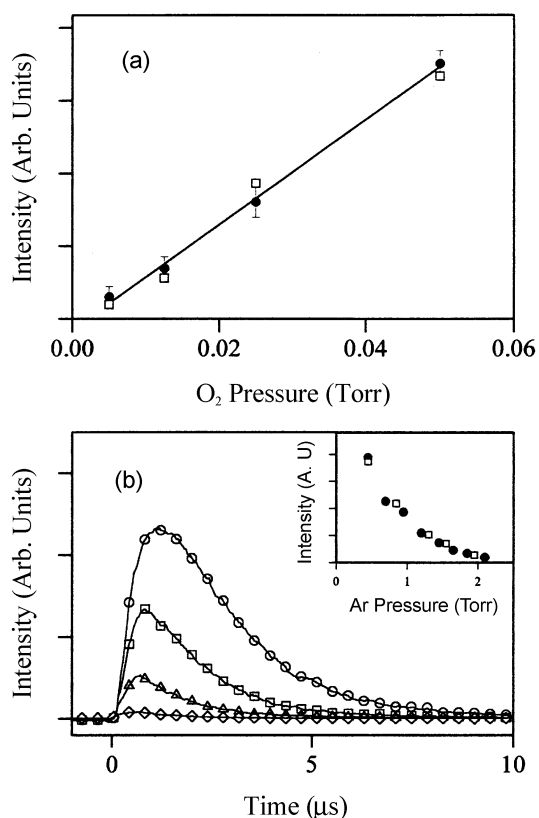
Figure 3. (a) Oxygen pressure dependence of CL intensities monitored at 400 (●) and 500 (□) nm, respectively. (b) Representative time profiles for the CL signal monitored at 400 nm vs. Ar buffer pressures: 0.45 (○), 0.95 (□), 1.45 (△), and 2.10 (◇) Torr of Ar. To avoid congestion, one data point from every 10 points is plotted. Time integrated CL intensities monitored at 400 (●) and 500 (□) nm vs. Ar pressure are shown in the insert of (b).
