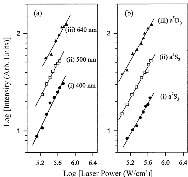
Figure 2. (a) Dependence of CL signal intensities on the photolysis laser power monitored at three different wavelengths. The magnitude of the slopes is (i) 2.1 \pm 0.2 , (ii) 2.0 \pm 0.2 , and (iii) 1.9 \pm 0.2 , respectively. (b) Dependence of LIF intensities for the low-lying atomic states of Cr atoms on the photolysis laser power. The magnitude of the slopes is (i) 1.8 \pm 0.2 , (ii) 1.9 \pm 0.2 , and (iii) 1.9 \pm 0.2 , respectively. To avoid congestion, plot (ii) and (iii) are vertically shifted.
