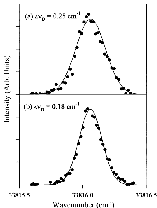
Figure 7. The z^5D_4 \leftarrow a^7S_3 absorption line profile at different delay time. The delay time between the photolysis and probe pulses was (a) 0 \mu\text{s} and (b) 5 \mu\text{s} . The Ar gas was slowly flowed over \text{Cr}(\text{CO})_6 powder at 273 K and the cell pressure was 2.0 Torr.
