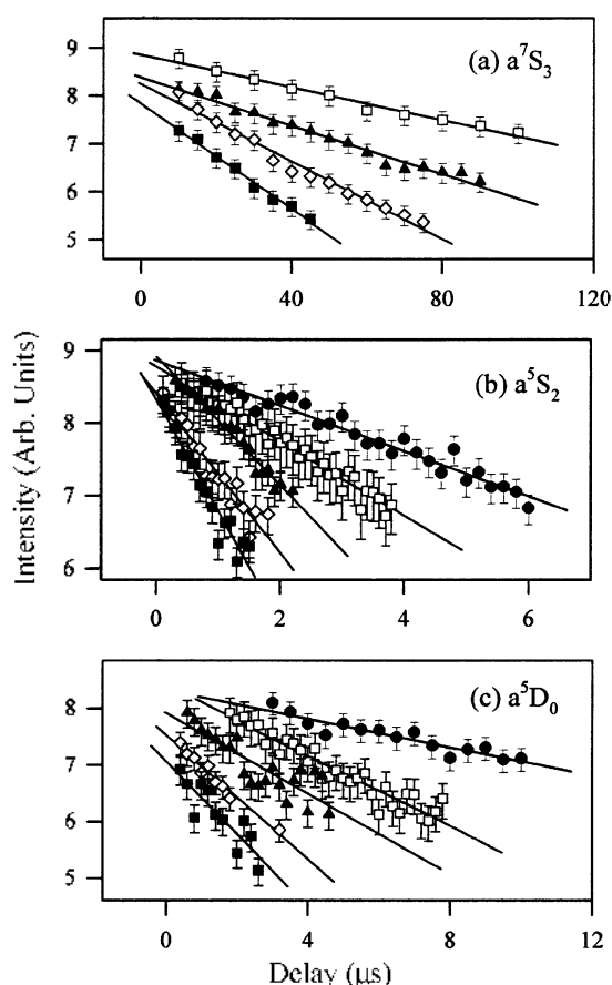
Figure 4. Dependence of LIF intensities of the low-lying atomic states of Cr atoms on the photolysis and probe delay time at different \text{O}_2 pressures. The partial pressures of \text{Cr}(\text{CO})_6 vapor and He were kept constant at 0.45 Torr. The partial \text{O}_2 pressures were (a) 0.25 ( \square ), 0.45 ( \blacktriangle ), 0.65 ( \nabla ), and 0.95 ( \blacksquare ) Torr. (b) 0.05 ( \bullet ), 0.25 ( \square ), 0.45 ( \blacktriangle ), 0.75 ( \nabla ), and 0.95 ( \blacksquare ) Torr. (c) 0.05 ( \bullet ), 0.25 ( \square ), 0.45 ( \blacktriangle ), 0.75 ( \nabla ) and 0.95 ( \blacksquare ) Torr, respectively.
