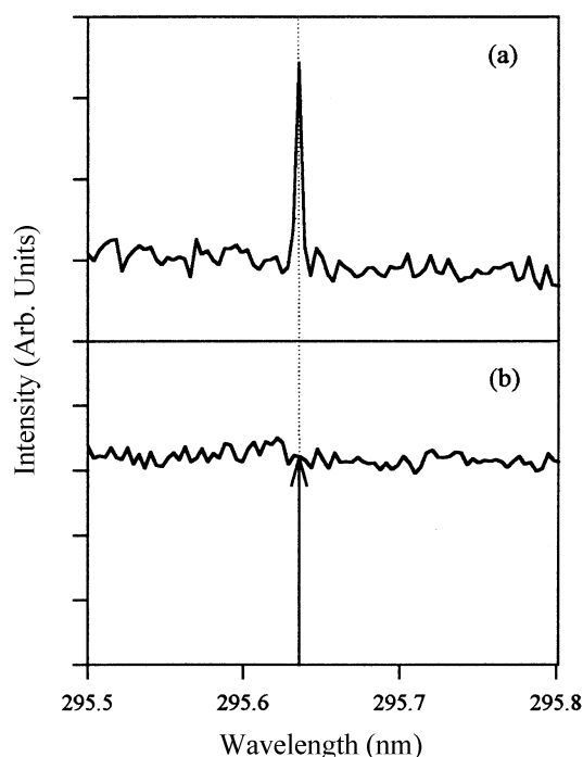
Figure 6. (a) Population change of \text{Cr}(a^5D_4) atoms by changing the photolysis laser wavelength. The probe laser frequency was set at z^5D_4^0 \leftarrow a^5D_4 transition (391.9 nm) and the fluorescence from z^5D_4^0 \rightarrow a^5D_3 transition was monitored at 388.8 nm. The delay time between photolysis and probe pulses was 2 \mu\text{s} . (b) Intensities of the CL signal monitored at 500 nm vs. photolysis laser wavelength. A 10% \text{O}_2 in He mixture was slowly flowed over \text{Cr}(\text{CO})_6 powder at 273 K and the total pressure in the cell was 0.5 Torr.
