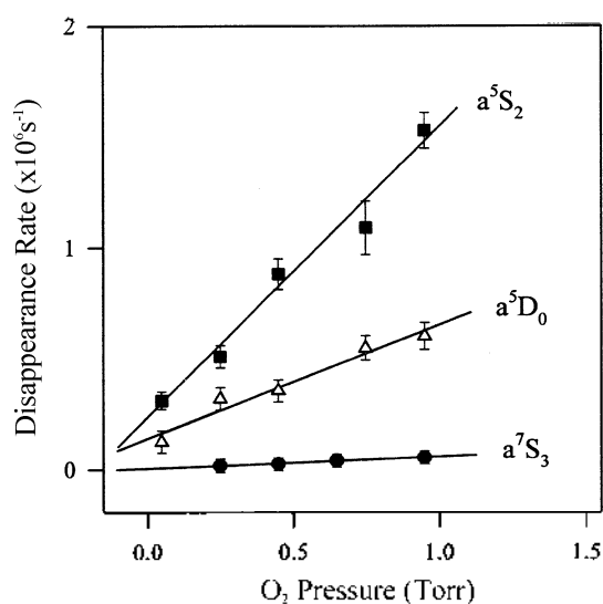
Figure 5. Oxygen pressure dependence of the disappearance rate for the low-lying atomic states of Cr atoms.
