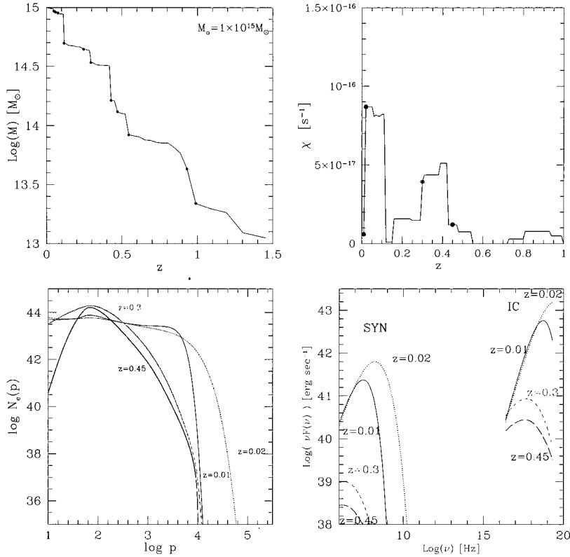
Fig. 3. — a) a single merger tree for a cluster with present-day mass of M_o = 1 \times 10^{15} M_\odot , each dot represents a merger event with M_2 \geq 10^{13} M_\odot ; b) the time-evolution (with redshift) of the electron acceleration coefficient ( \tau_{acc} = \chi_{acc}^{-1} ) during the cluster formation; c) the evolution of the electron spectrum at different relevant times (see panel) in the same cluster; d) the corresponding radio (synchrotron) and hard-X ray (IC) emission. Calculations are performed assuming: R_H = 500h_{50}^{-1} Kpc , \eta_t = 0.26 , \eta_e = 0.003 and \langle B \rangle = 0.5 \mu G .
