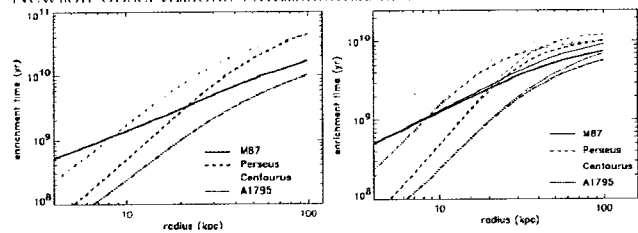
Fig. 17. — Enrichment ages of the central iron abundance peak in the four galaxy clusters, M87/Virgo, Centaurus, Perseus, and A1795. The enrichment times were calculated on the basis of a SN Ia rate of 0.15 SNU (Capellaro et al. 1999) and an additional contribution by stellar mass loss. Left panel: with constant SN Ia rate, Right panel: with increasing SN Ia rate in the past described by a power law with time exponents s = -2 (thick lines) and s = -1.1 (thin lines).
