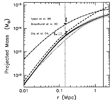
Fig. 6. — Projected mass profile of the cluster CL0024+17 (thick line) from XMM-Newton observations compared to strong gravitational lensing results (Zhang et al. 2004a).
