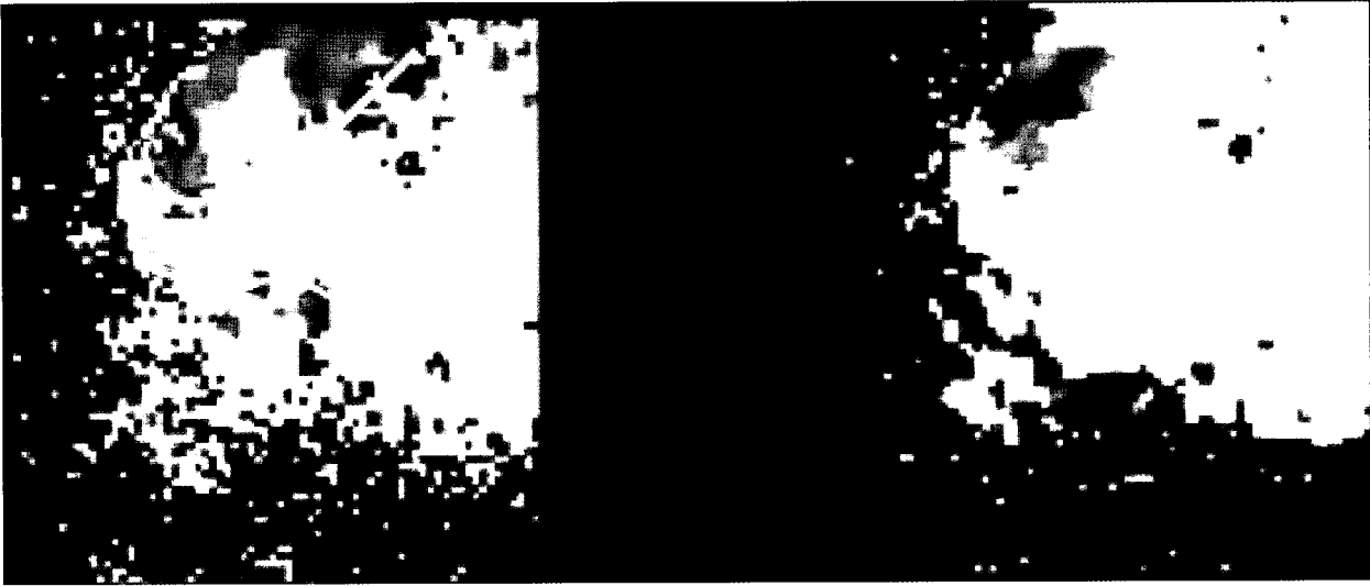
Fig. 2.— Polarization of the eastern lobe of Cygnus A, original and derived maps kindly provided by C. Carilli & R. Perley – these maps were derived from multifrequency data at 3.7cm using the VLA. Left: Magnetic field orientation, color coded; Right: Rotation Measures (arbitrary color scale). Hand-drawn white lines indicate positions where rapid shifts in magnetic field direction are accompanied by rapid shifts in Rotation Measure – an unambiguous signature of rotation measure local to the source, not due to any intervening cluster field.
