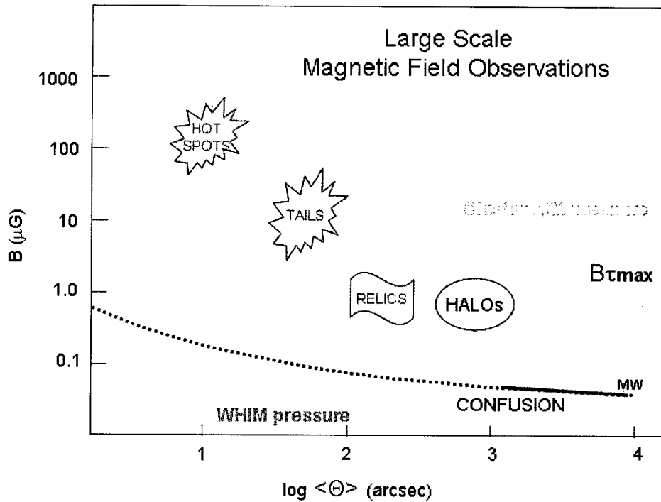
Fig. 1.— [B, \theta] space - a perspective on observed structures, pressure-equivalent benchmarks, and observational constraints. The curved dashed line towards the bottom represents the confusion limit, irreducible in the large angle (solid line) portion due to the Milky Way.
