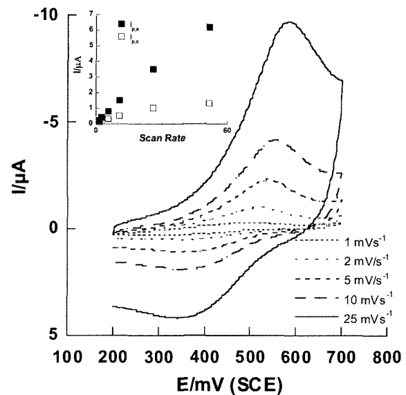
Fig. 4. Cyclic voltammogram of LCCI fungal laccase on the 2,2'-dithiosalicylic aldehyde-modified a gold flag electrode as a function of scan rate; 0.2 M citrate-phosphate buffer (pH 5.85), 25°C. The linear dependence of cathodic and anodic peak currents ( i_{p,c} and i_{p,a} ) to scan rate ( \nu ) is shown in the inset. Anaerobic conditions were maintained by purging a single-compartment cell with nitrogen gas during the each measurement.
