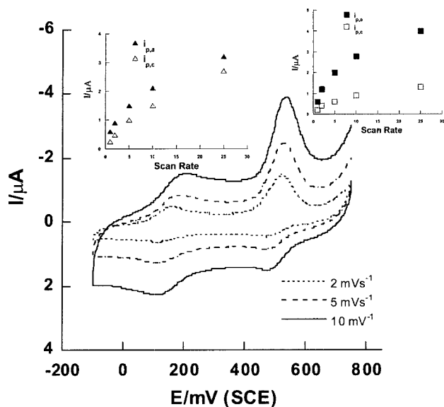
Fig. 5. Cyclic voltammogram of LCCIIa fungal laccase on the 2,2'-dithiosalicylic aldehyde-modified a gold flag electrode as a function of scan rate; 0.2 M citrate-phosphate buffer (pH 5.85), 25 °C. The linear dependence of cathodic and anodic peak current to scan rate ( \nu ) is shown in the insets. Anaerobic conditions were maintained by purging a single-compartment cell with nitrogen gas during the each measurement.
