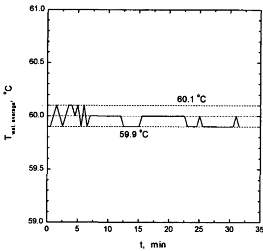
Fig. 4. Changes in the Average Water Temperature
