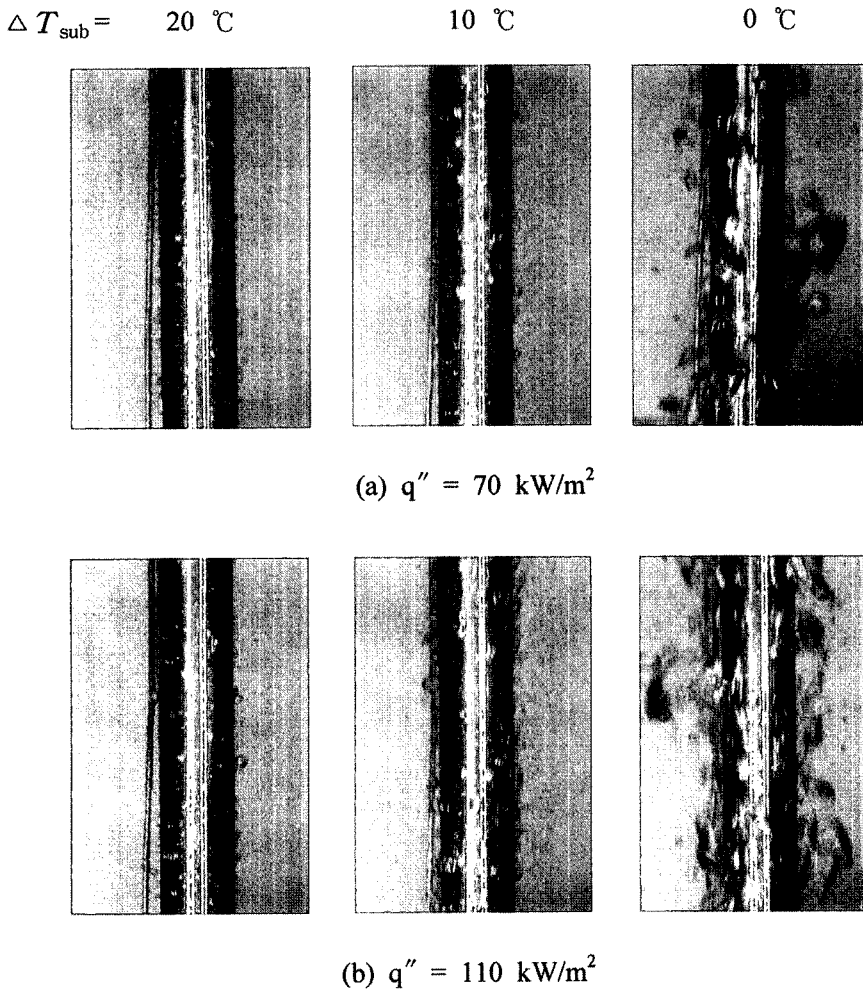
Fig. 8. Photos of Subcooled Boiling on the Unrestricted Single Tube Surface
