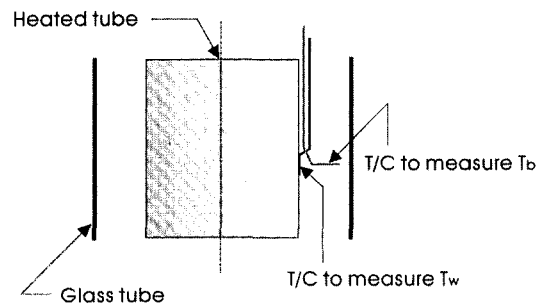
Fig. 2. Locations of Thermocouples in the Annulus
