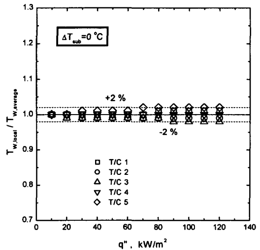
Fig. 5. Comparison Local Wall Temperatures with Average Values in the Annulus
