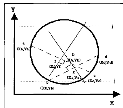
Fig 2. Tracking position extraction for iris edge
