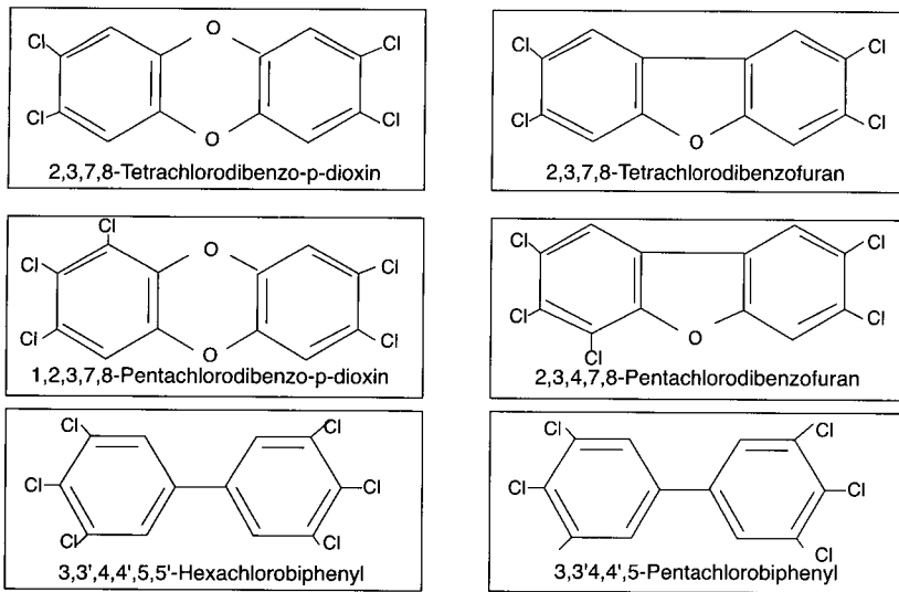
Figure 1. Chemical structure of dioxin and related compounds.
