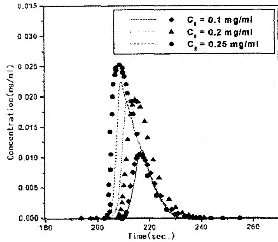
Fig. 4. Comparison of experiments and calculated values at different concentration of caffeine with a=7.45, b=2.1 of Langmuir isotherm parameters; mobile phase flow rate=0.7 ml/min., sample loading amount=20 μl, wavelength=254 nm.
