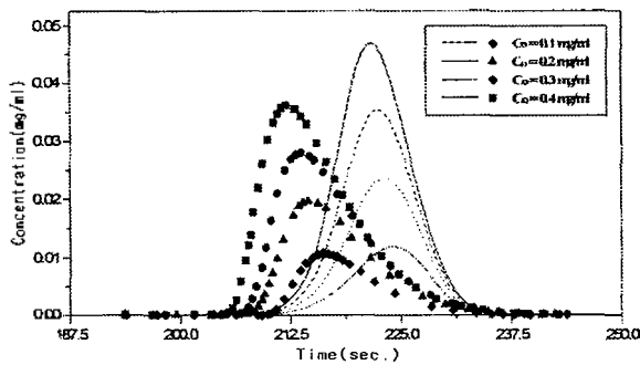
Fig. 2. Comparison of experiments and calculated values at different concentration of caffeine with a=4.44, b=0.19 of Langmuir isotherm parameters; mobile phase flow rate=0.7 ml/min., sample loading amount=20 μl, wavelength=254 nm.
