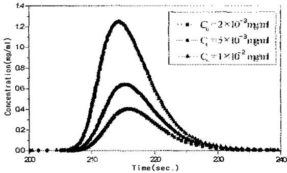
Fig. 1. Chromatograms of experiments at different concentration of caffeine; mobile phase flow rate=0.7 ml/min., sample loading amount=20 μl, wavelength=254 nm.
