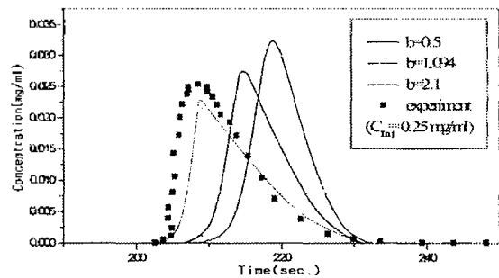
Fig. 3. Comparison of experiments and calculated values at different Langmuir isotherm parameter b with a=7.45; mobile phase flow rate=0.7 ml/min., sample loading amount=20 μl, wavelength=254 nm.
