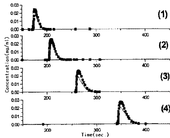
Fig. 5. Chromatograms of experiments and calculated at different flow rate of mobile phase ; sample loading amount=20 μl, wavelength=254 nm, wavelength=254 nm, mobile phase flow rate: (1)=0.8 ml/min, (2)=0.7 ml/min, (3)=0.5 ml/min, (4)=0.4 ml/min.
