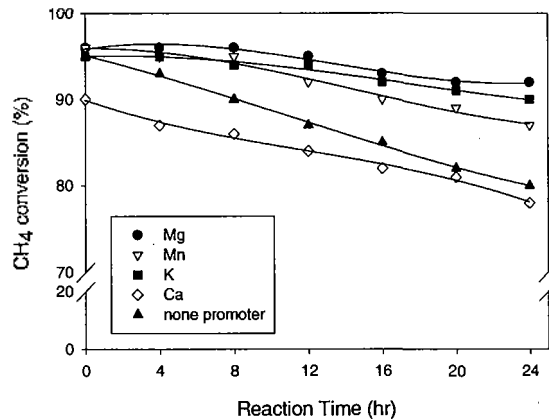
Fig. 5 CH 4 conversion over promoters added 13wt% Ni/HY-zeolite catalyst for 24hr reaction (reaction temperature=700°C).
