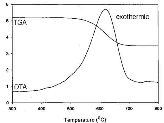
Fig. 11. TGA and DTA diagrams of coke-deposited 13wt%Ni/HY-zeolite catalyst after 24hr reaction at 700°C : heating rate = 10°C/min in air.
