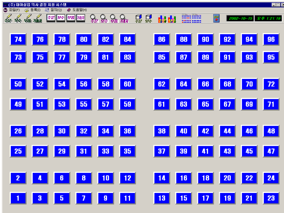
FIGURE 4. User interface
