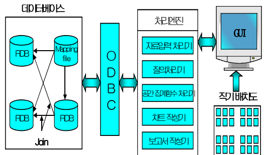
FIGURE 3. System architecture
