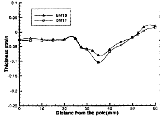
Fig. 5 Comparison of the thickness strain between BHF 10ton and BHF 11ton (square cup, horizontal direction stroke=30mm, aluminum)
