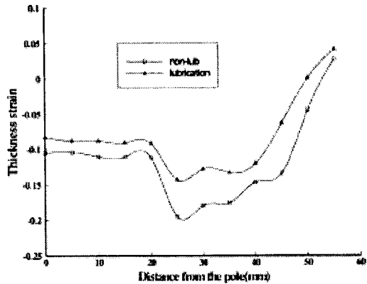
Fig. 7 Comparison of thickness strain between lubrication and non-lubrication.(cylinder cup, BHF 12ton, stroke=40mm, steel)
