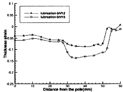
Fig. 6 Comparison of the thickness strain distribution between BHF 12ton and BHF 15ton (square cup, diagonal direction, stroke=30mm, steel)
