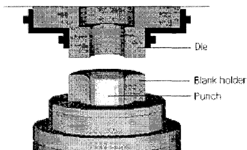
Fig. 2 Cross-sectional view of geometric description of the tooling for deep drawing
