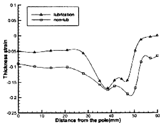
Fig. 9 Comparison of the thickness strain between lubrication and non-lubrication. (square cup, BHF 14ton, diagonal direction, stroke=30mm, steel)
