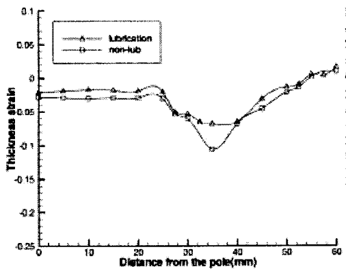
Fig. 8 Comparison of the thickness strain between lubrication and non-lubrication. (square cup, BHF 11ton, horizontal direction, stroke=30mm, aluminum)
