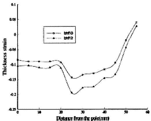
Fig. 4 Comparison of the thickness strain distribution between the BHF 10ton and BHF 12ton (cylinder cup, radial direction, stroke=40mm, steel)
