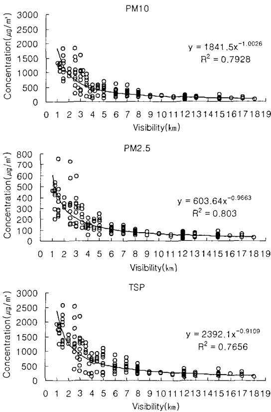
Fig. 3. Distribution of dust concentrations and visibility during Sand storm events in Seoul (2002)
