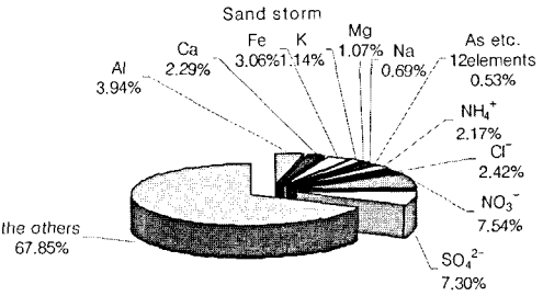
Fig. 5. Average chemical composition of PM 10 during sand storm period and normal period in Seoul Area.
