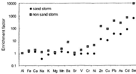
Fig. 4. Enrichment factor of heavy metals in PM 10
