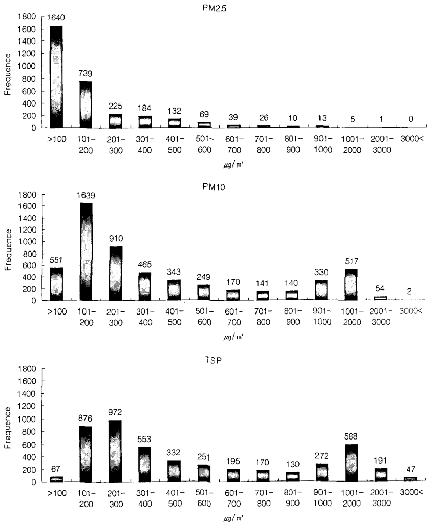
Fig. 2. Sand storm frequencies observed in Seoul (2000~2002)
