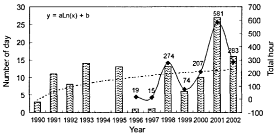
Fig. 1. Sand storm events in Seoul during 1990-2002.
