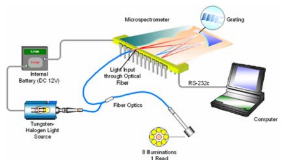
Fig. 1. Schematic diagram of the portable NIR system.
