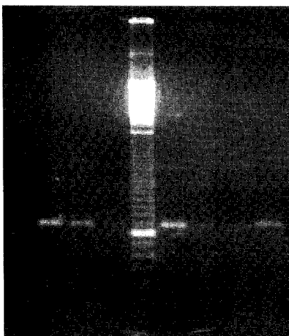
Fig. 2. Agarose gel electrophoresis of products of PCR amplification using primers NS3 and NS6. A single product of 907 bp was produced in all isolates tested. HITO = laboratory strain, M = marker.
