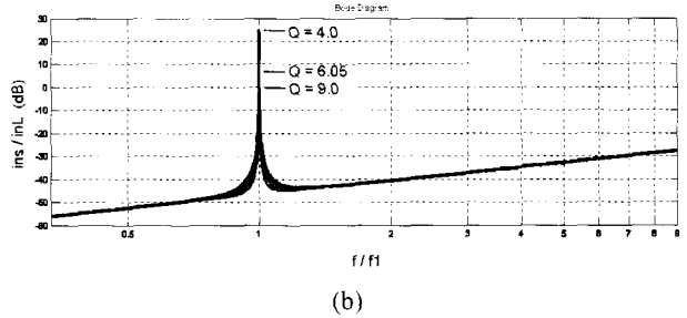
Fig. 3. Block diagram and compensation characteristics of the conventional control method: (a) block diagram of the closed loop control system and (b) compensation characteristics.
