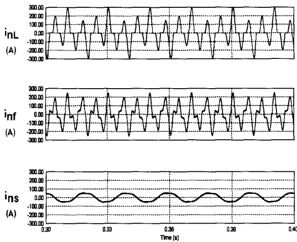
Fig. 6. Simulated waveforms of the proposed control method.
