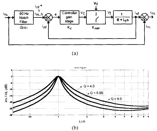
Fig. 5. Block diagram and compensation characteristics of the proposed control method: (a) block diagram of the closed loop control system and (b) compensation characteristics.
