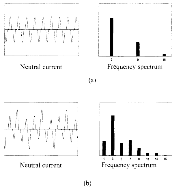
Fig. 1. Neutral current waveform: (a) balanced load condition and (b) unbalanced load condition.
