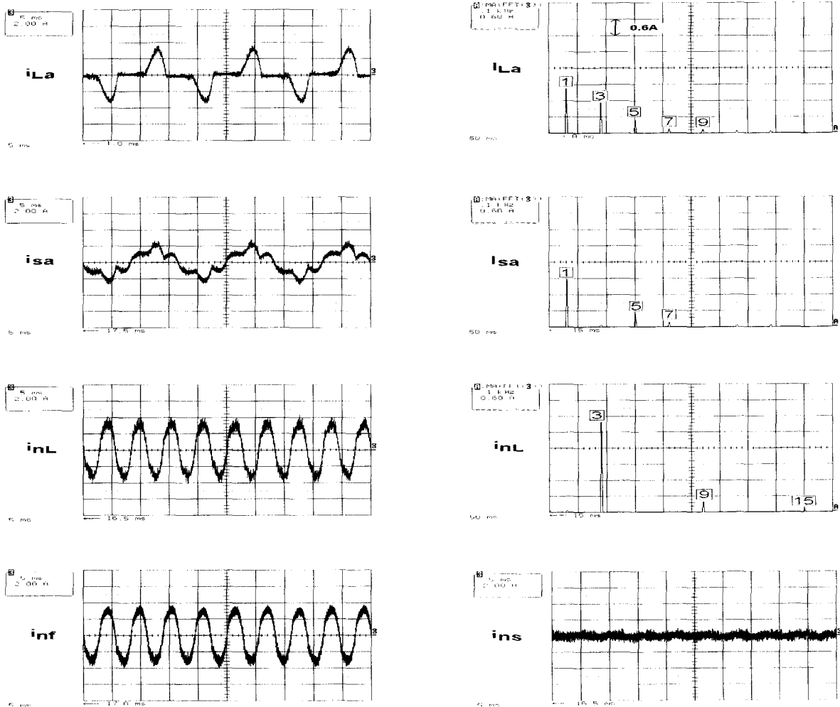
Fig. 7. Experimental waveforms and frequency spectra under balanced loading (2A/div, 5ms/div).
