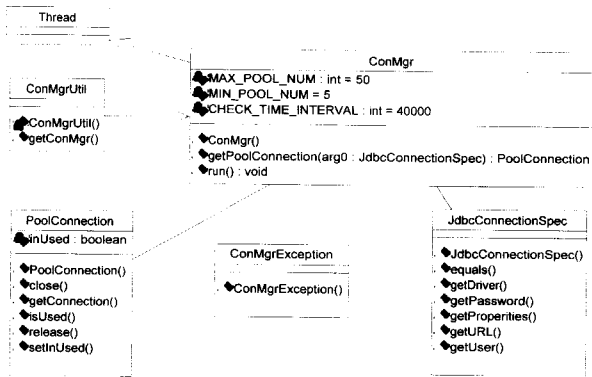
(그림 11) DB Connection Pool Class Diagram
