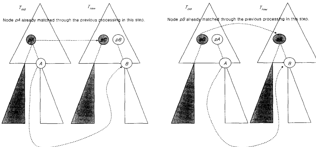
(a) Case A in the algorithm
