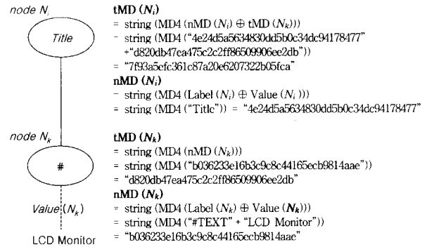
(Figure 4) An example of Node_MD and Tree_MD
