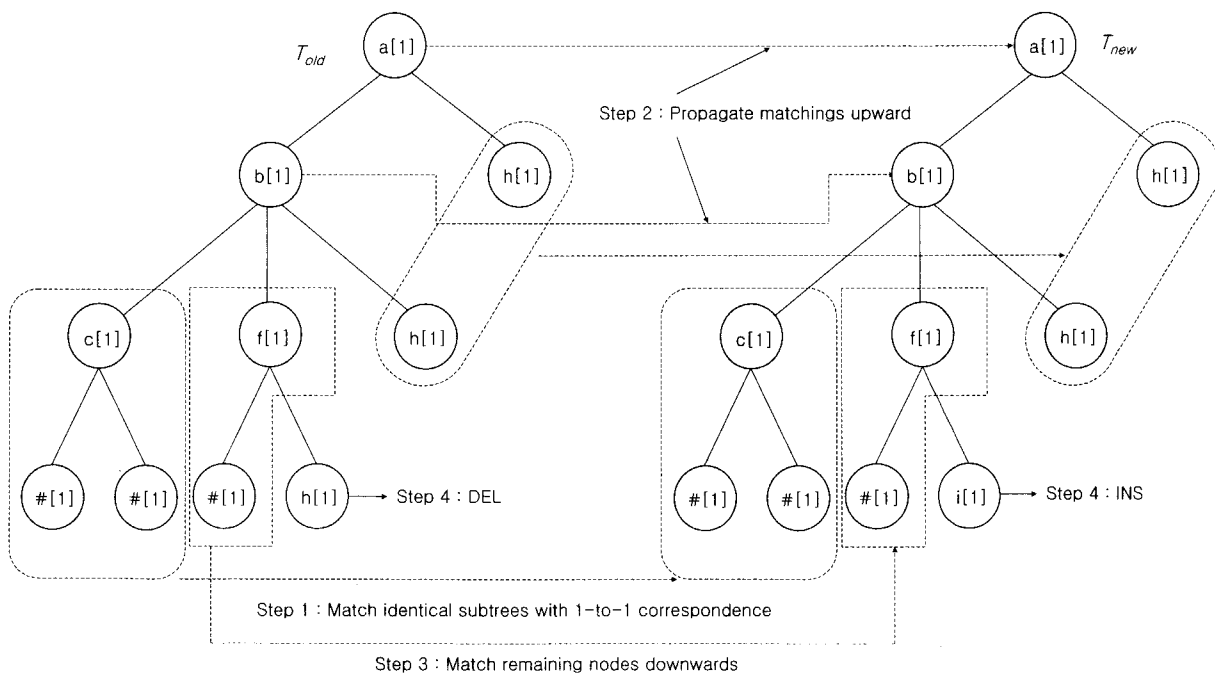
(Figure 5) Illustration of X-tree Diff algorithm
