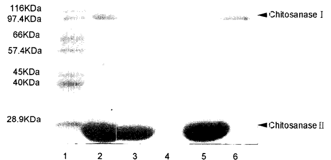
Fig. 4. 12% SDS-PAGE analysis of chitosanases during protein purification steps. Lane 1: size marker, Lane 2: crude enzyme, Lane 3: DEAE cellulose active fraction pool, Lane 4: S-Sepharose active fraction pool A1, Lane 5: S-Sepharose active fraction pool A2 (used as chitosanase II), Lane 6: Superdex 75 HR 10/30 active fractions (used as chitosanase I).
