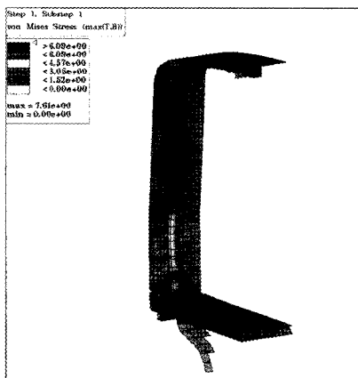
Fig. 3 Stress distribution at bonding parts between the composite front end and the Al car body
