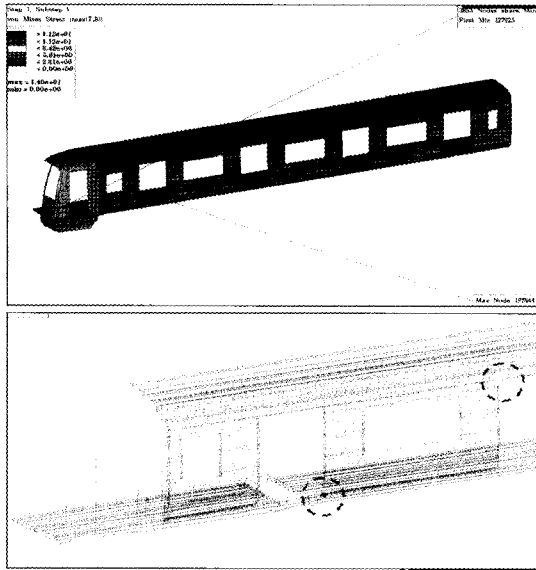
Fig. 2 Stress distribution under the normal loading condition
