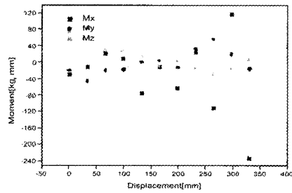
Fig. 4 Distribution of force and moment for the compressive load condition
