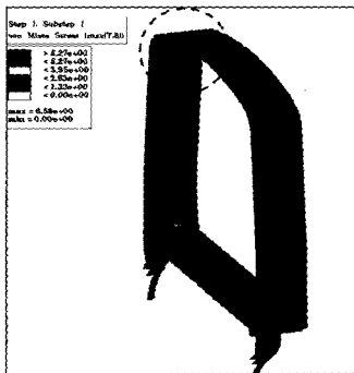
Fig. 6 Stress distribution for the torsional load condition
