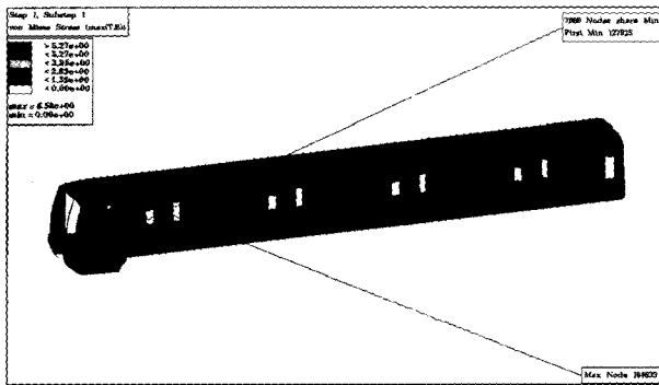
Fig. 6 Stress distribution for the torsional load condition(continued)
