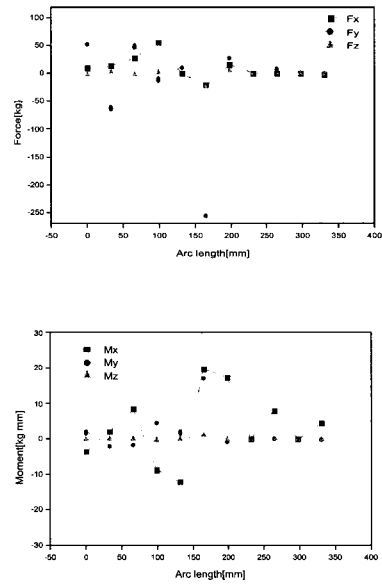
Fig. 9 Distribution of force and moment for the compressive load condition
