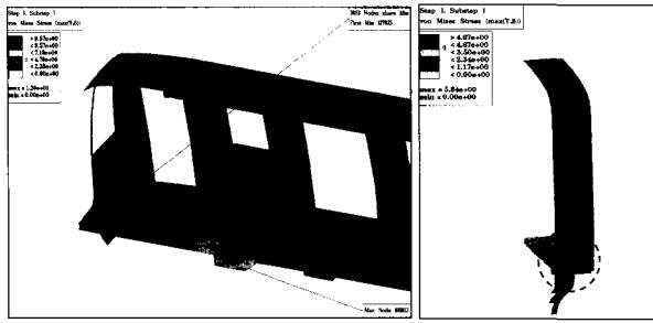
Fig. 8 Bonding parts for the compressive load condition
