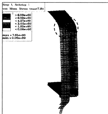
Fig. 3 Stress distribution at bonding parts between the composite front end and the Al car body(continued)
