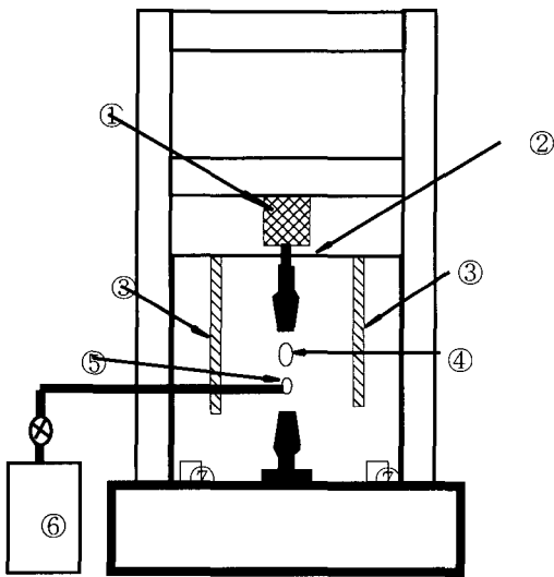
Fig. 2. Schematic diagram of experimental apparatus. ① load cell ② chamber ③ heating coil ④ thermocouple ⑤ injection nozzle ⑥ nitrogen bombe ⑦ fan
