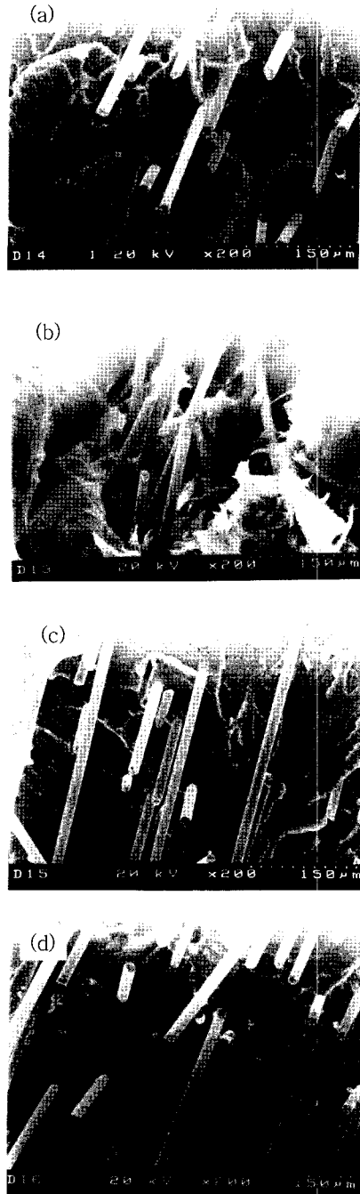
Fig. 5. SEM photographs of tensile fracture surfaces for 10% fiber fraction at various temperature. (a) R.T., (b) 60°C, (c) -15°C, (d) -50°C
