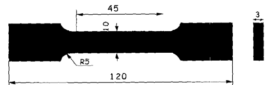
Fig. 1. Specimen geometries for tensile test (unit : mm).
