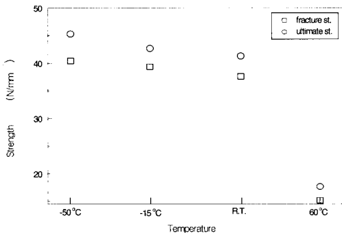
Fig. 4. Ultimate strength and fracture strength for various temperature.
