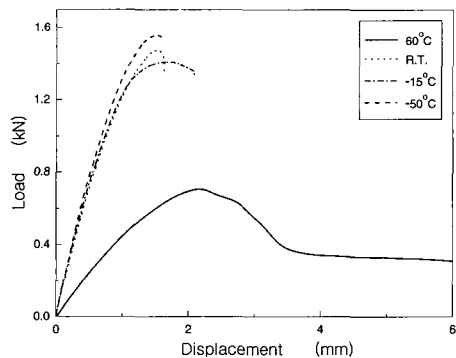
Fig. 3. Load-displacement curves at various temperature.
