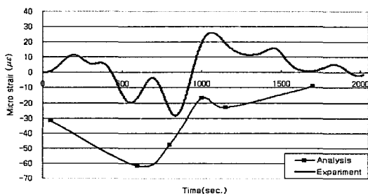
Fig. 14 Comparison between measurement and analysis results(second stress concentration point: vertical direction)
