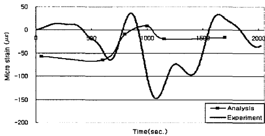
Fig. 13 Comparison between measurement and analysis results(first stress concentration point: vertical direction)
