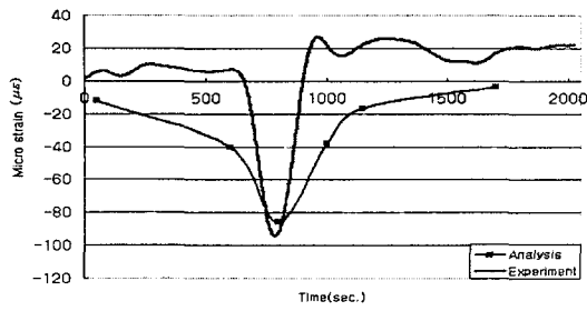
Fig. 11 Comparison between measurement and analysis results(general point)
