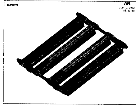
Fig. 6 FE model of ladle crane using shell elements
