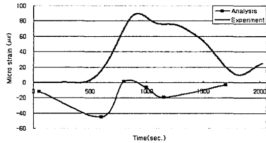
Fig. 12 Comparison between measurement and analysis results(first stress concentration point: horizontal direction)
