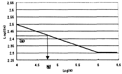
Fig. 17 Remaining fatigue life calculation using S-N curve
