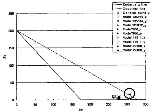
Fig. 16 Assessment results considering residual stress
