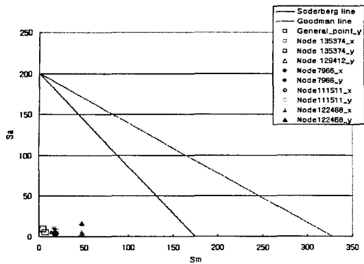
Fig. 15 Assessment results using fatigue diagram(SS400)
