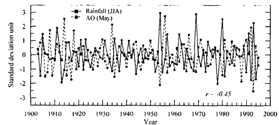
Fig. 2. Time-series of May AO index and summer monsoon rainfall over Yangtze River valley and southern Japan. Shown as the results from a high-pass filter, through which the variations longer than 10 years are removed.
