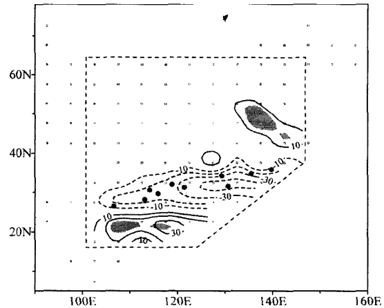
Fig. 1. Changes in summer precipitation (mm) corresponding to a one standard deviation of the May AO index for the period 1900-1998. Grey squares indicate the grids with data availability above 95% in the entire period. Regions above 95% confidence level are shaded. Ten stations are shown as filled circles. Contour interval is 10mm. Zero contours are omitted.
