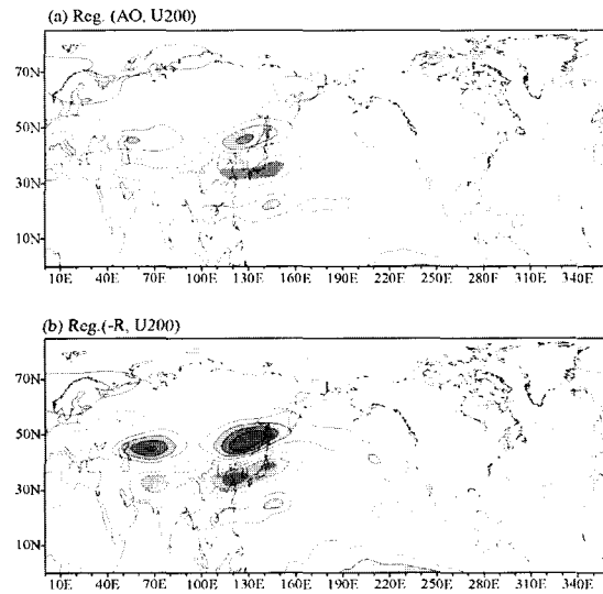
Fig. 3. Changes in summer zonal wind ( \text{m s}^{-1} ) at 200 hPa associated with a one standard deviation anomaly in the May AO index (a) and in the simultaneous ten-station-mean rainfall for summer (b) for the period 1958-1999. To facilitate comparison rainfall records are multiplied by -1. The contour interval is 0.5 \text{ m s}^{-1} per standard deviation of May AO and summer rainfall, respectively. Zero contours are omitted. Regions below -0.5 \text{ m s}^{-1} and above +0.5 \text{ m s}^{-1} are shaded.
