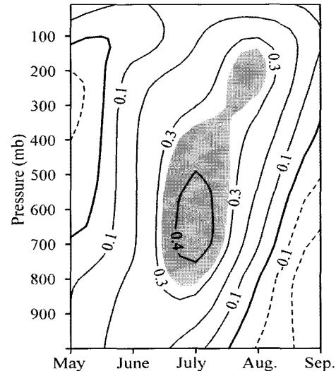
Fig. 5. Cross correlation between the May AO index and the regional averaged geopotential height over the domain 100°E-160°E and 30°N-40°N. Values exceeding the 95% confidence level are shaded.
