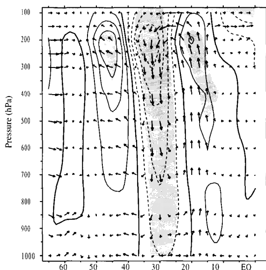
Fig. 4. Cross section of the zonal mean zonal wind ( u ), meridional wind ( v ) and vertical motion ( w ) over East Asia (110°-150°E) regressed onto the May AO index. The u is shown as the contours with interval of 0.3 \text{ m s}^{-1} . Zero lines are bold and easterly are shown in dashed lines. Regions above 95% confidence level are shaded. The covariance of v and w are shown as vectors. Values are \text{m s}^{-1} (for u and v ) and \text{hPa s}^{-1} (for w ), corresponding to a one standard deviation anomaly in the May AO index. Before regression the AO index are normalized. The values of largest vectors are 0.47 \text{ m s}^{-1} for v and 4.310^{-3} \text{ hPa s}^{-1} for w .
