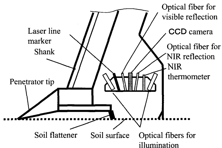
Fig. 2 Soil penetrator and sensor probes arrangement.
