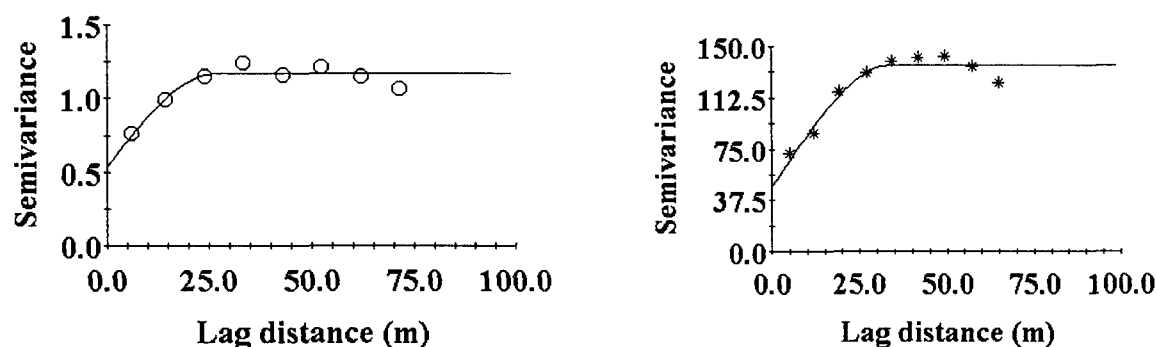
Fig. 4 Semivariograms of SOM content (left) and NO 3 -N content (right) of a 0.5 ha paddy field.
