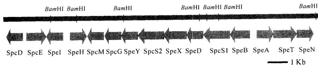
Fig. 1. Organization of gene cluster for spectinomycin biosynthesis, and speculated gene products.
