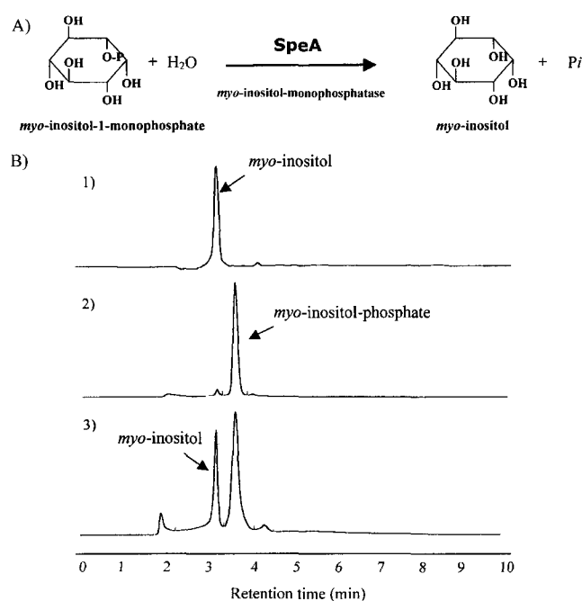
Fig. 3. SpeA catalyzes the formation of myo -inositol from myo -inositol-1-phosphate. (A) Incubation of myo -inositol-1-P with cell extract of speA expressed in E. coli produced myo -inositol. (B) HPLC analysis of the reaction products. The myo -inositol, a product of SpeA activity, was detected by HPLC. 1) myo -inositol standard. 2) Reaction with cell extract harboring only pET28a plasmid. 3) Reaction with cell extract harboring speA gene. All reactions were stopped after 30 min of incubation.
