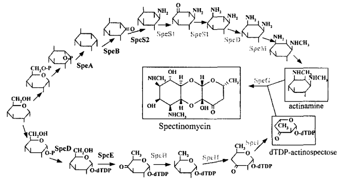
Fig. 6. The proposed biosynthetic pathway of spectinomycin based on the deduced functions of the isolated gene products.
