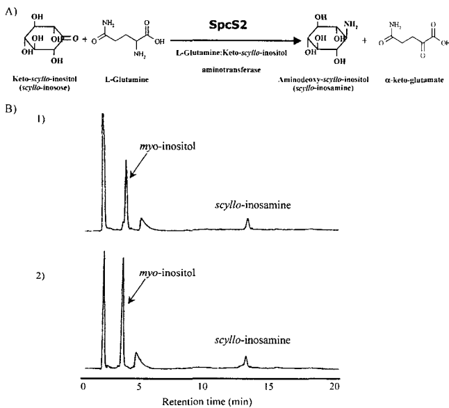
Fig. 5. Sps2 functions downstream of SpeB in the biosynthetic pathway of spectinomycin. (A) Sps2, sps2 product is proposed to be L-glutamine:scyllo-inositol aminotransferase. (B) HPLC analysis of the reaction products. The scyllo -inosamine, the reaction product of Sps2, was detected by HPLC. 1) Reaction product with cell extracts containing SpeB and Sps2. 2) Reaction product with commercial myo -inositol-dehydrogenase and cell extract containing Sps2. All reactions were stopped after 60 min of incubation.
