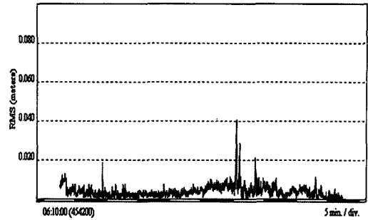
Fig. 9 RMS of RTK GPS after post-processing
