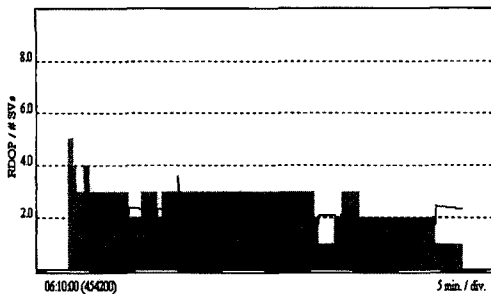
Fig. 8 RDOP of RTK GPS after post-processing
