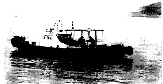
Fig. 10 Equipment tsetting for bathymetric survey
