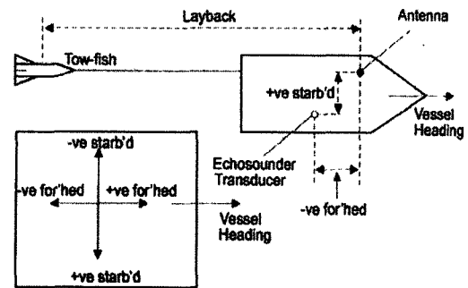
Fig. 11 Vessel offsets
