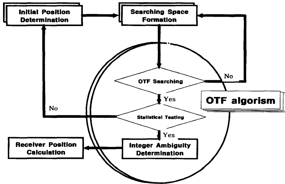
Fig. 2 Flow-chart of the OTF
