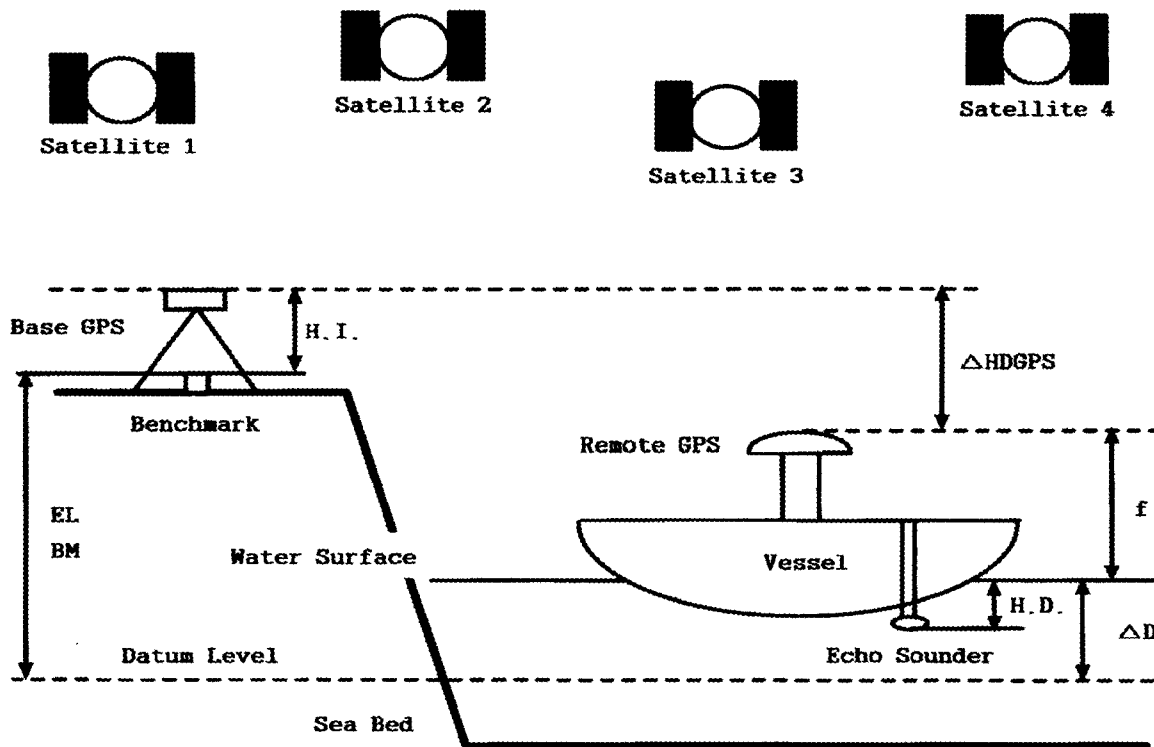
Fig. 3 RTK GPS water's surface elevation measurement technique
