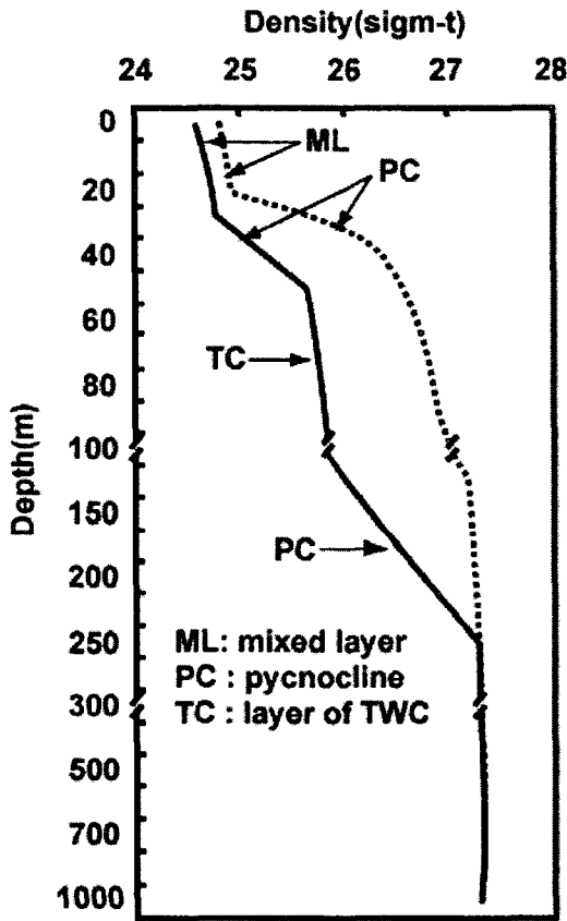
Fig. 9. Vertical profile of density gradient at st.1 (dashed line) and st.4 (solid line) of line A.
