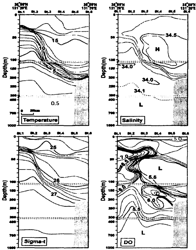
Fig. 4a. Vertical section of temperature (°C), salinity (psu), sigma-t and dissolved oxygen (ml/l) along line A in June, 1996.
