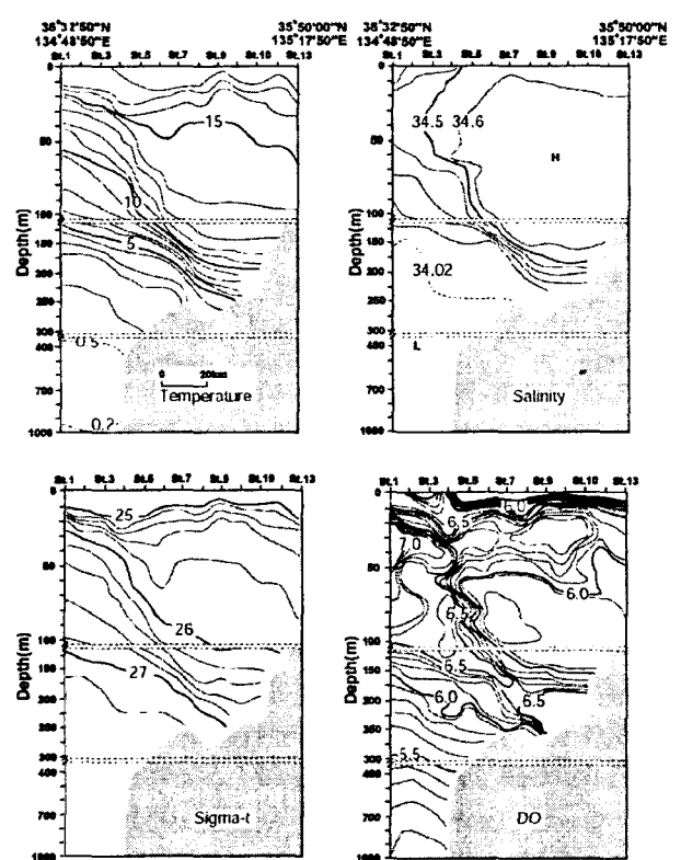
Fig. 4d. Continued along line D.
