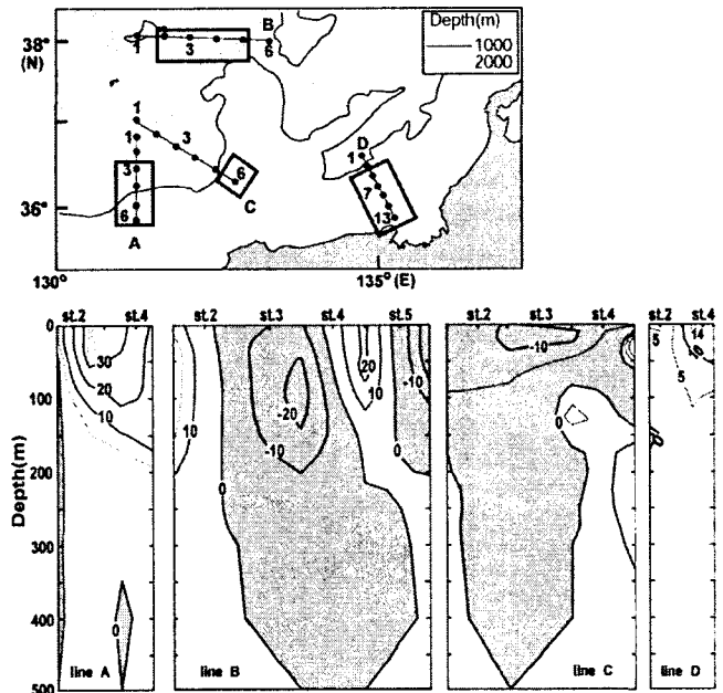
Fig. 8. - Top: study area (rectangles indicate regions where high salinity greater than 34.6psu exists), - Bottom : vertical section of geostrophic currents (cm/sec) along each observation lines (shade areas represent flows out of paper).
