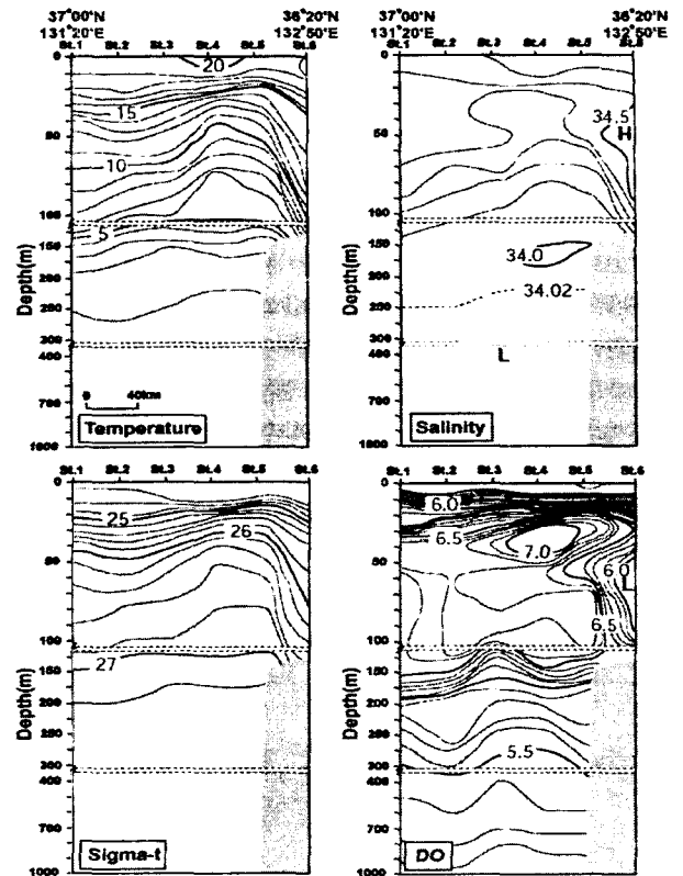
Fig. 4c. Continued along line C.
