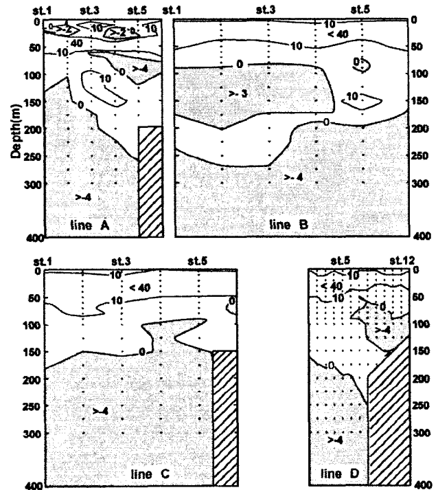
Fig. 10. Vertical section of Brunt Vaisala frequency ( \times 10^{-6} \text{ sec}^{-1} ) along each observation line in June, 1996. Shaded areas represent layers less than zero.
