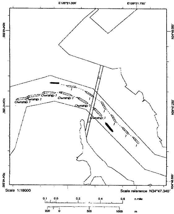
Fig 4 Trace of ship's passage under Bridge
