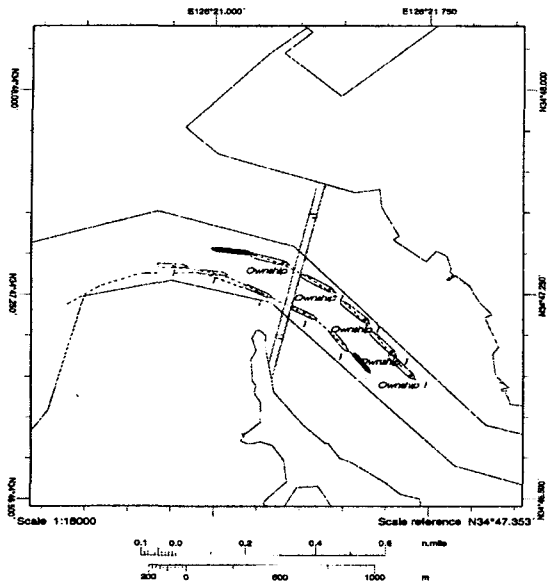
Fig 5 Trace of ship's passage under Bridge
