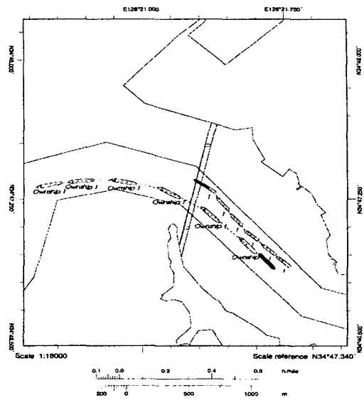
Fig 3 Trace of ship's passage under Bridge
