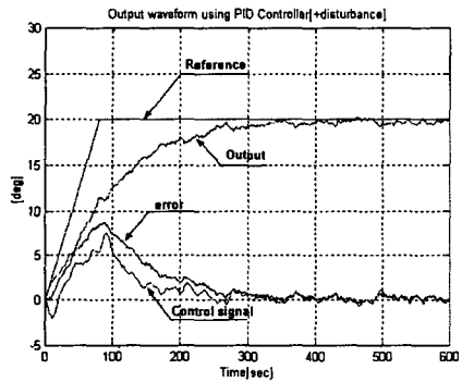
(b) (+) 외란 (b) (+) disturbance
