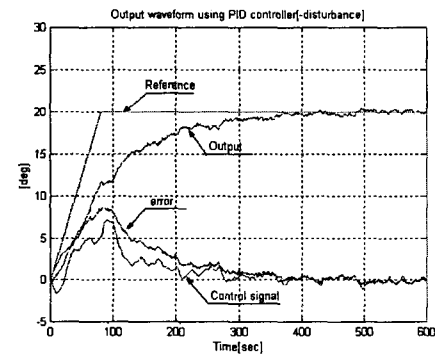
(c) (-) 외란 (c) (-) disturbance
