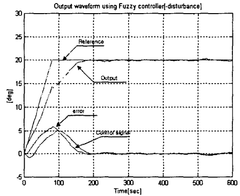
(b) (+) 외란 (b) (+) disturbance
