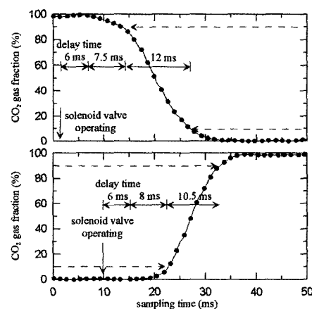
Fig. 9 Measurement of system response with operating solenoid valve at gas flow rate 2.5 l/min, \Delta P=0.5 bar, span gas ( \text{CO}_2 ) 20%, zero gas ( \text{N}_2 ) 99.999%
