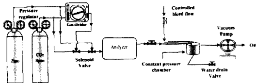
Fig. 3 Schematic diagram of test equipment for calibration and system response measurement of FRNDIR
