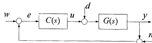
Fig. 6 Weighting schemes for closed-loop performance
