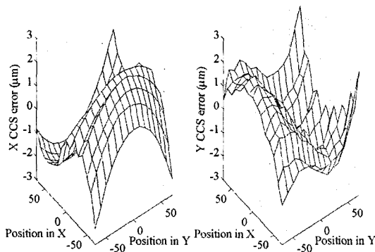
Fig. 3 Linearity errors of the front 8-segment CCS
