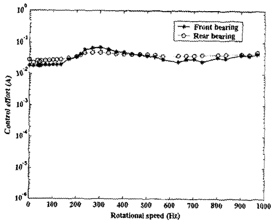
(b) The \mu control
