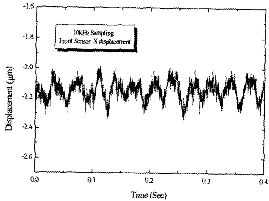
Fig. 17 Stationary suspension noise of the CCS
