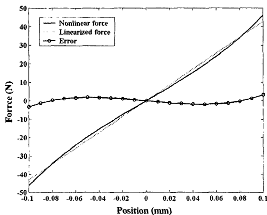
Fig. 1 The linearity error of open-loop stiffness
