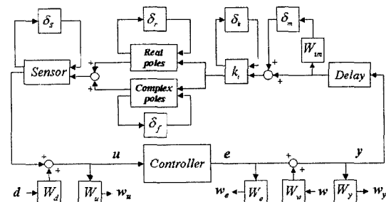
Fig. 8 Block diagram of the augmented plant
