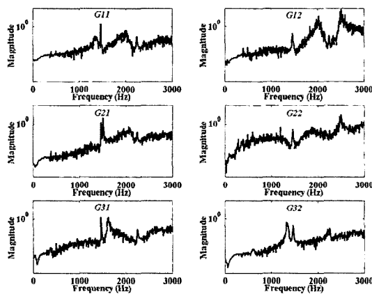
Fig. 4 Relative deviation of measured frequency responses
