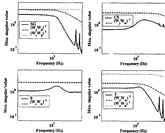
Fig. 12 Weighting functions and measured closed-loop frequency responses
