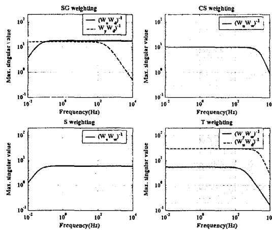
Fig. 7 Performance weighting functions
