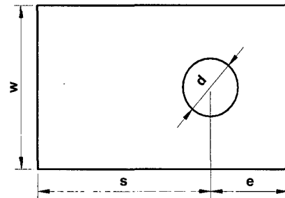
(b) Rectangular edge[R, S]
