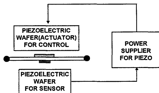
Fig. 5 Three major parts of the control equipment
