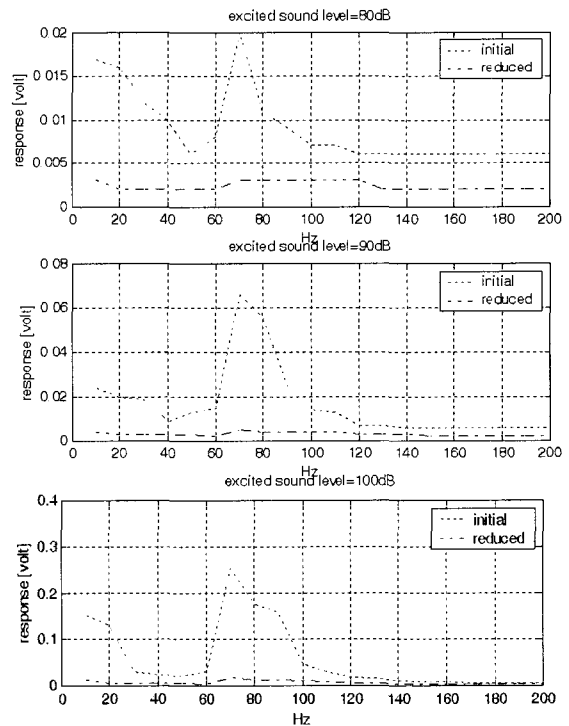
Fig. 8 Comparison of the responses with and without the piezoelectric actuator (aspect ratio = 2.0)
