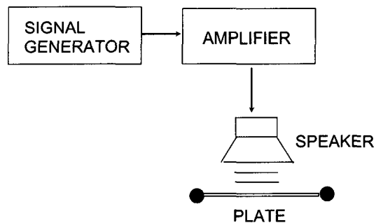
Fig. 4 Acoustic equipment
