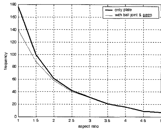
Fig. 1 Ball joint and piezoelectric sensor and actuator effect for the frequency responses at different aspect ratio
