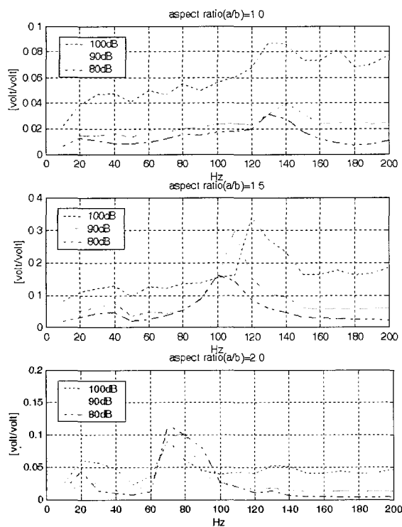
Fig. 7 Comparison of normalized response of piezoelectric sensor to the sound excitation
