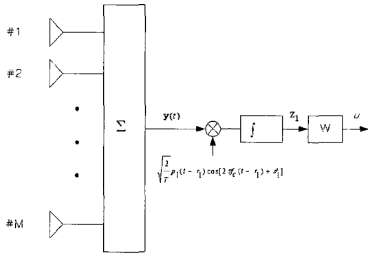
Fig. 2 CDMA reverse link adaptive array receiver model.
