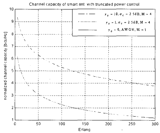
Fig. 5 Normalized channel capacity.
