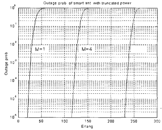
Fig. 4 Outage probability versus Erlang capacity ( \sigma_c = 2.5 dB, \gamma_0 = 1 ).
