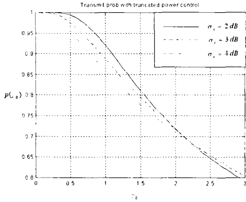
Fig. 1 Transmit probability of a mobile station ( m=4 ).
