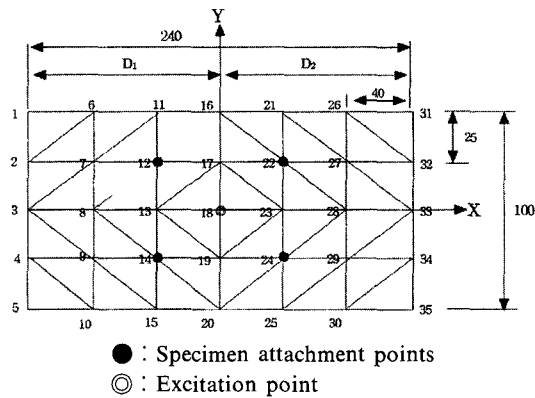
Fig. 1 Original plate fixture model
