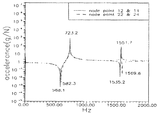
Fig. 2 FRF of original plate fixture model
