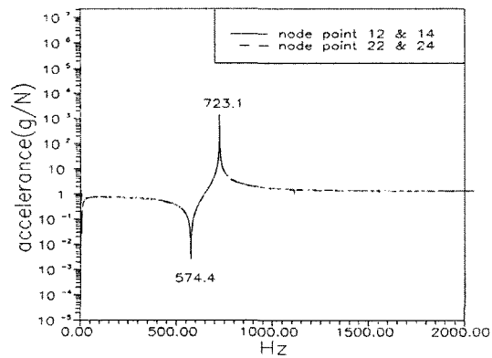
Fig. 6 FRF after thickness modification
