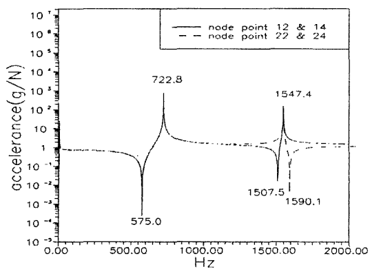
Fig. 4 FRF after length modification
