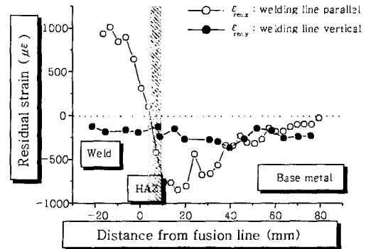
Fig. 8 Saw-cutting results(strain)
