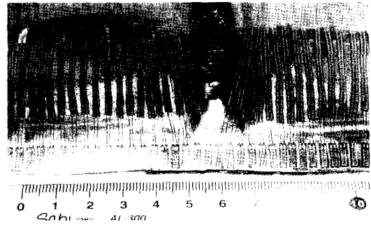
Fig. 6 Specimen used in saw-cutting test
