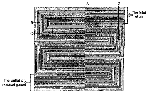
(b) The air flow channel configuration on flow-field plate
