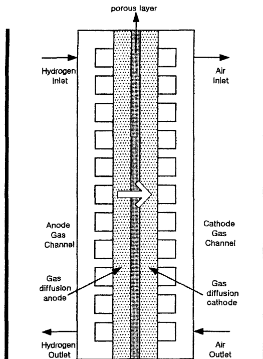
Fig. 3 Schematic diagram of a PEMFC
