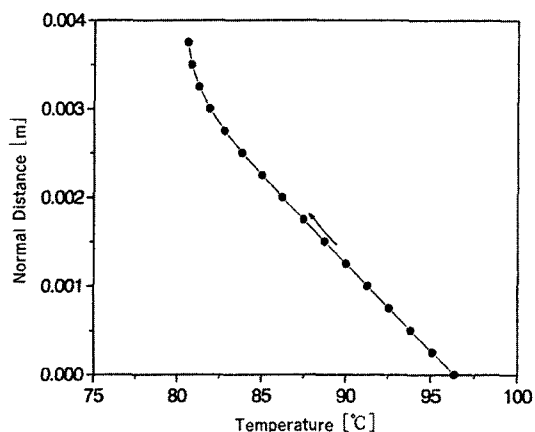
Fig. 14 Temperature distribution along normal section, B-B
