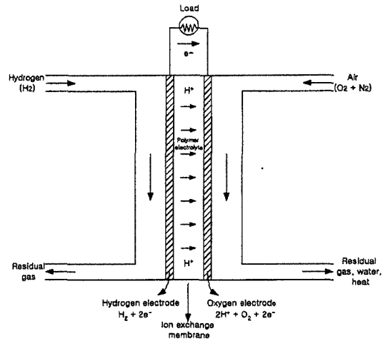
Fig. 1 Schematic of an individual fuel cell (Adopted from Fuel Cell Hand Book, 2000)
