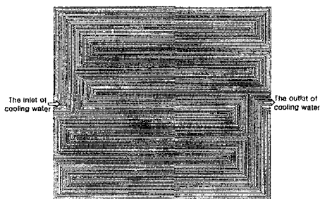
(c) The cooling water flow channel configuration on flow-field plate
