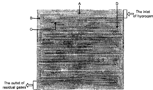
(a) The hydrogen flow channel configuration on flow-field plate
