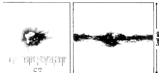
Fig. 11 Impacted CAI specimen (a) before and (b) after CAI strength test showing compression failure with a kink-band shear([45/-45/0/90] 3s - IM7/8552).
