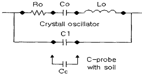
Fig. 3 Equivalent circuit of the crystal oscillator and moisture sensor.
