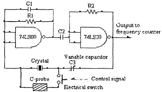
Fig. 4 Circuit diagram of the oscillator.
