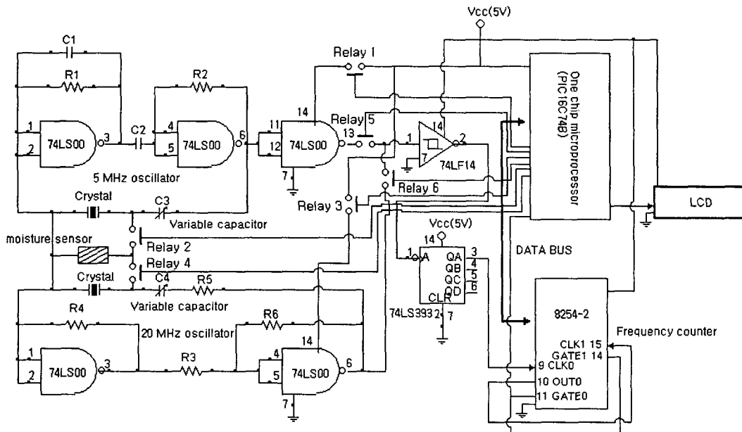
Fig. 5 Circuit diagram of the oscillators with sensor and signal processing unit.
