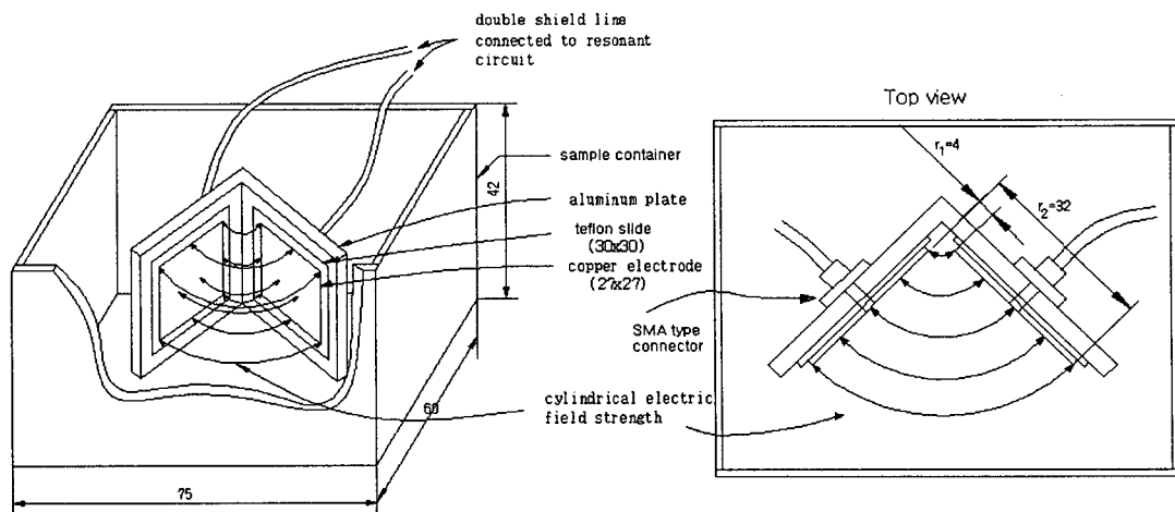
Fig. 2 Schematic view of the perpendicular plate type moisture sensor and sample container.
