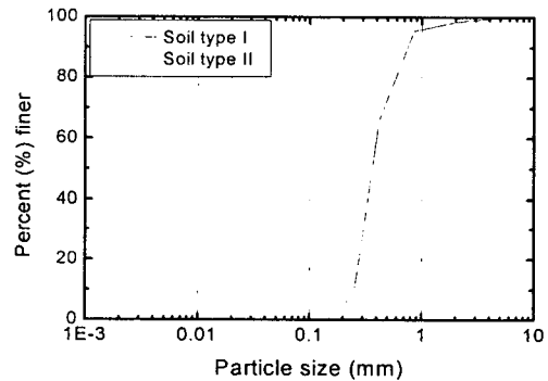
Fig. 1 Grain size distributions of soil samples.
