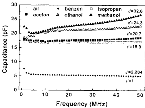
Fig. 6 Capacitance changes of the moisture sensor with several standard dielectrics.
