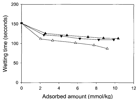
Fig. 4. Wetting time of PET fabrics dyed with Dye-6-22(△), Dye-8-22(▼), and Dye-10-22(▲).
