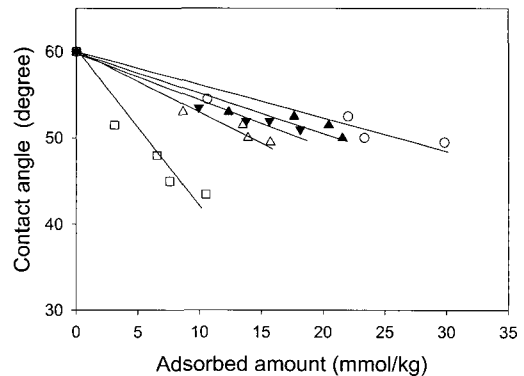
Fig. 2. Water contact angle on PET film treated with Dye-6-13(○), Dye-6-22(△), Dye-6-45(□), Dye-8-22(▼), and Dye-10-22(▲).
