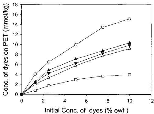
Fig. 1. Dye uptakes of PET fabric dyed for 60 minutes at liquor to fiber ratio of 80:1; Dye-6-13(○), Dye-6-22(△), Dye-6-45(□), Dye-8-22(▼), Dye-10-22(▲).
