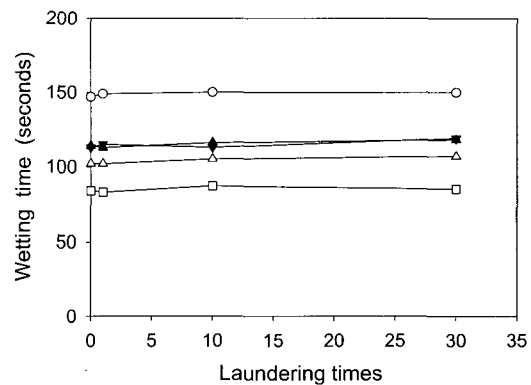
Fig. 5. The effect of laundering on the wetting time of PET fabrics dyed with Dye-6-13(○), Dye-6-22(△), Dye-6-45(□), Dye-8-22(▼), and Dye-10-22(▲).
