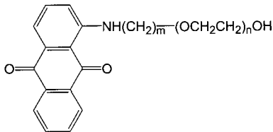
Scheme 1. Structure of 1-(6-ethoxylated alkylamino)anthraquinone.
