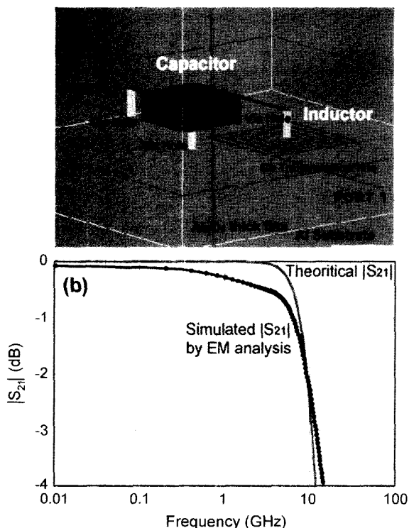
Fig. 7. (a) 3-dimensional structure of 10 GHz low pass filter consisted of a spiral-type inductor and a \text{Ba}(\text{Mg}_{1/3}\text{Ta}_{2/3})\text{O}_3 (BMT) microwave capacitor and (b) theoretical and simulated transmission characteristics.
