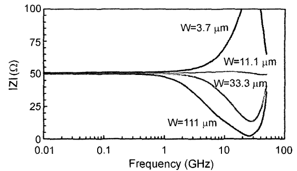
Fig. 5. Dependence of the characteristic impedance with the variation of the width of copper lines on aerosol-deposited Al 2 O 3 thick films.
