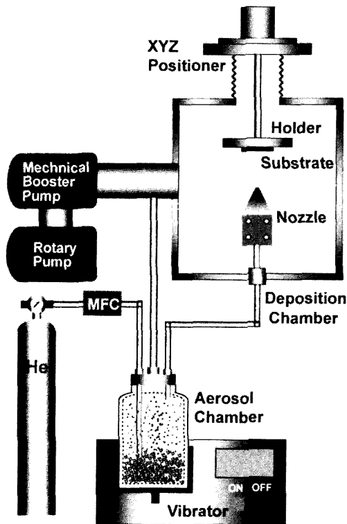
Fig. 1. Schematics of the aerosol deposition apparatus.
