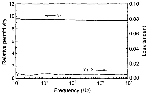
Fig. 4. Frequency dependence of the relative permittivity and loss tangent of aerosol-deposited Al 2 O 3 thick films.
