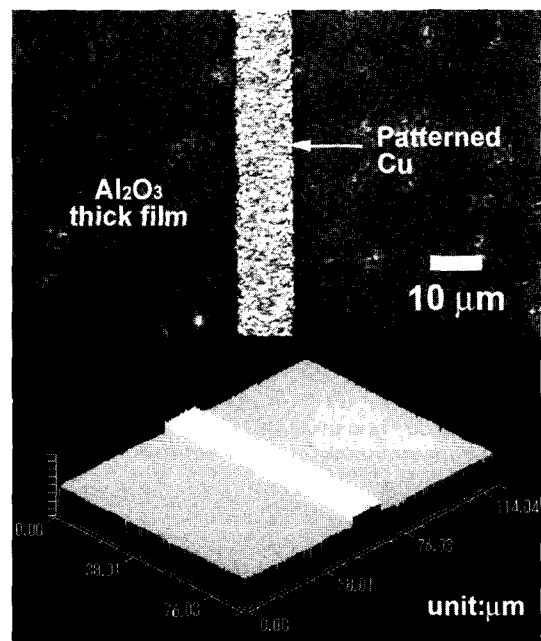
Fig. 6. Laser microscope images of a microstrip line formed on aerosol-deposited Al 2 O 3 thick films by copper electroplating.
