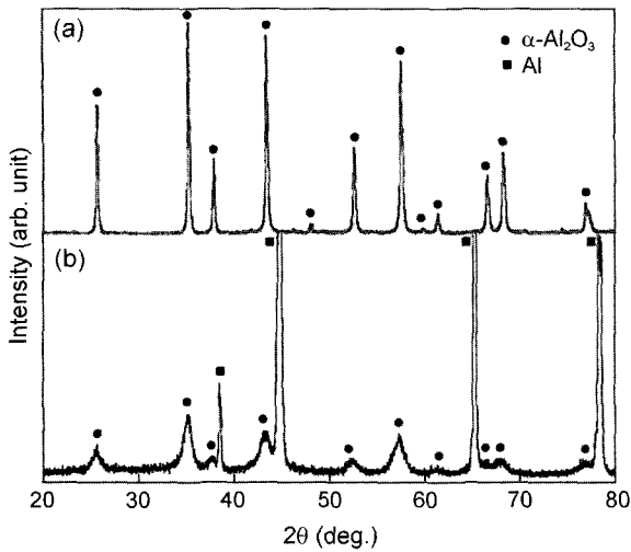
Fig. 3. X-ray diffraction patterns of (a) Al 2 O 3 powders (SG160B) and (b) aerosol-deposited Al 2 O 3 thick films on Al substrates at room temperature using SG160B powders.
