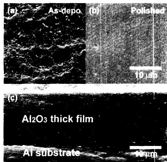
Fig. 2. Plane-view SEM micrographs of (a) as-deposited, (b) polished, and (c) a cross-sectional SEM micrograph of \text{Al}_2\text{O}_3 thick films on Al substrates at room temperature.
