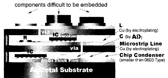
Fig. 8. Proposal of new RF modules by embedding both active and passive components using AD process.
