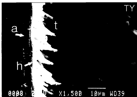
Fig. 5. TY group showing 1.5 µm thick hybrid layer (h) and numerous resin tags (t) which were 5-10 µm long and dense. (SEM ×1,500)
