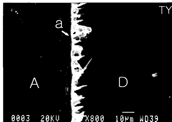
Fig. 4. Dentin (D) and Aelitefil (A) interface showed close adaptation and 5 µm thick adhesive layer (a) in Tyrian SPE (TY) group. (SEM ×800)
