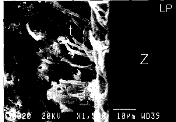
Fig. 8. LP group showing short and long resin tags (t) which were 5-15 µm long. (SEM ×1,500)
