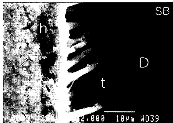
Fig. 2. SB group showing 2-4 µm thick hybrid layer (h) with taper resin tags (t) which were 10 µm long and had regular interval. (SEM ×2,000)
