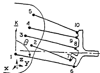
Fig. 2 The multi-link five-point suspension with the assigned points
