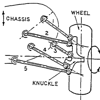
Fig. 1 The multi-link five-point suspension system
