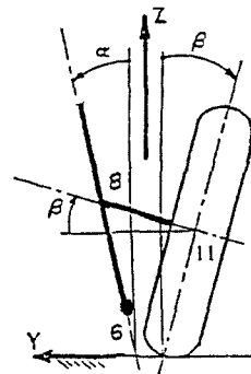
Fig. 3 Kingpin and camber angles
