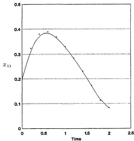
Fig. 4 Time (s) variation of z_{11} (m)
