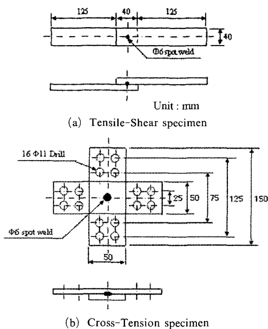
Fig. 1 Configuration of the spot-welded specimen
