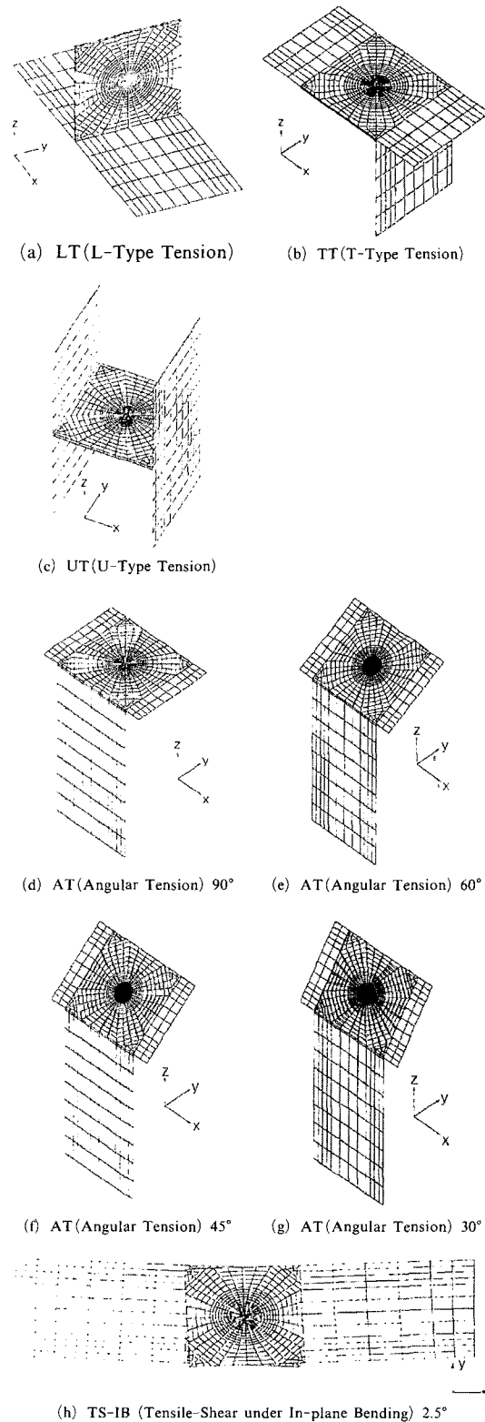
Fig. 8 FEM models of various spot-welded joints
