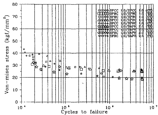
Fig. 7 Transformed relationship of Von Mises stress and fatigue life
