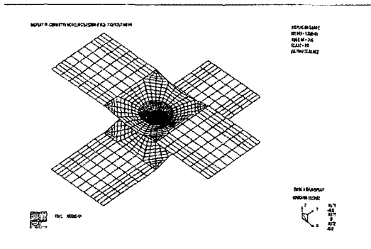
(b) Cross-Tension SPCC 1.0/SPCC 1.0 specimen
