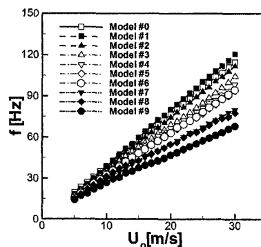
Fig. 2 Variation of vortex shedding frequency
