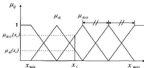
Fig. 2. MF definition before tuning (genetic optimization).
