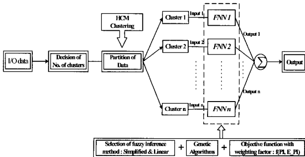
Fig. 3. Multi-FNN structure and ensuing development environment.
